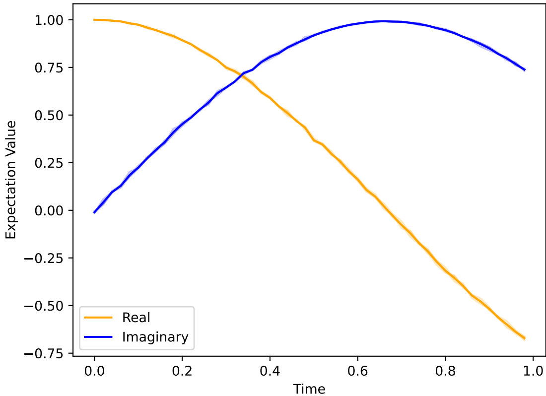
Expectation Value with \Delta t=0.02
