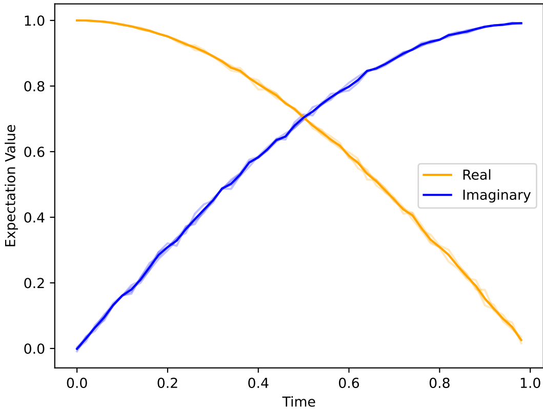
Expectation Value with \Delta t=0.02
