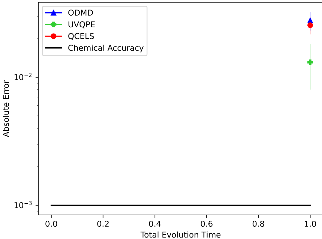
Convergence Absolute Error in Energy for TFI
