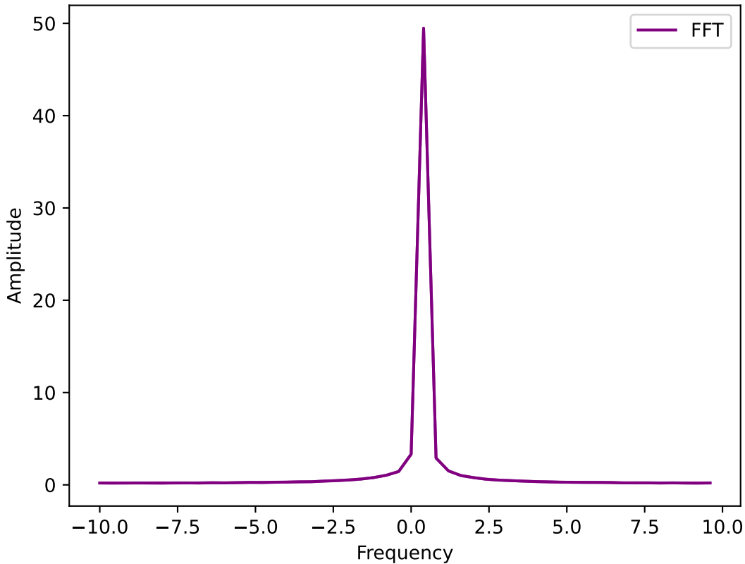
Fourier Transform of Expectation Value with \Delta t=0.05
