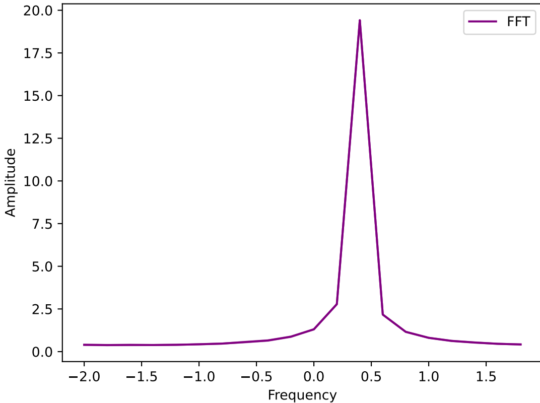
Fourier Transform of Expectation Value with \Delta t=0.25
