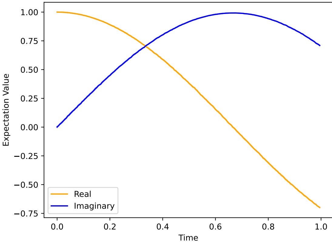
Expectation Value with \Delta t=0.005
