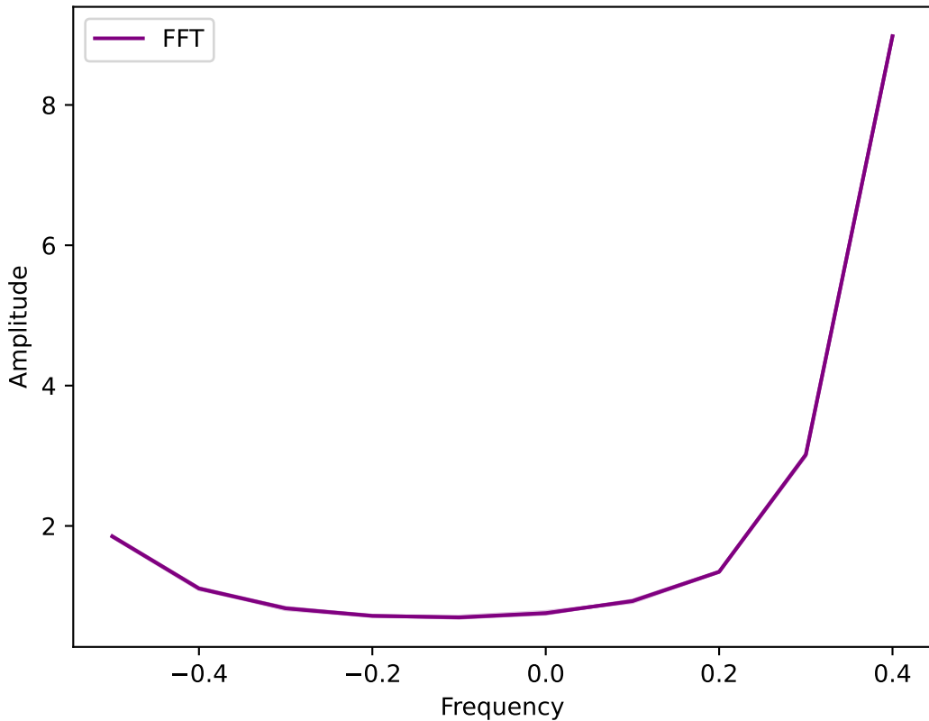
Fourier Transform of Expectation Value with Dt=1.0
