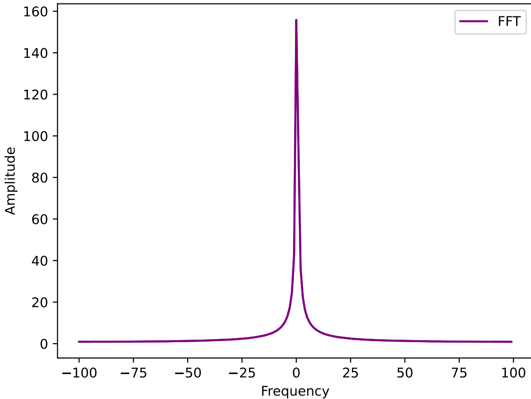
Fourier Transform of Expectation Value with \Delta t=0.005
