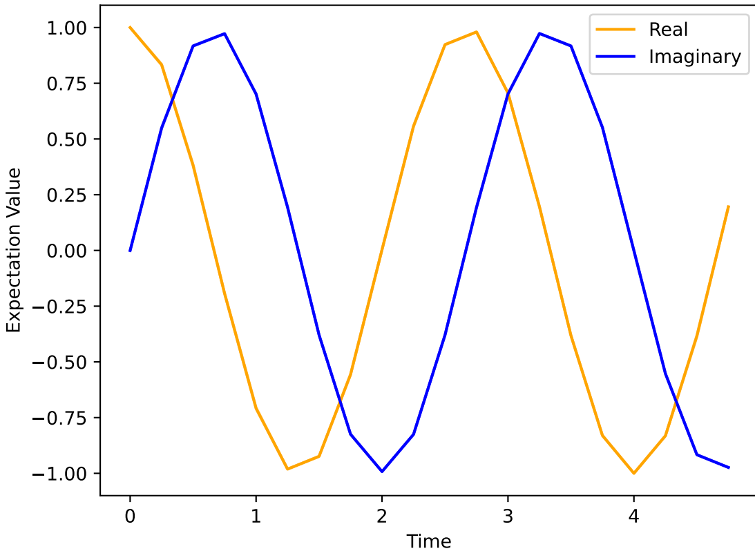
Expectation Value with Dt=0.25
