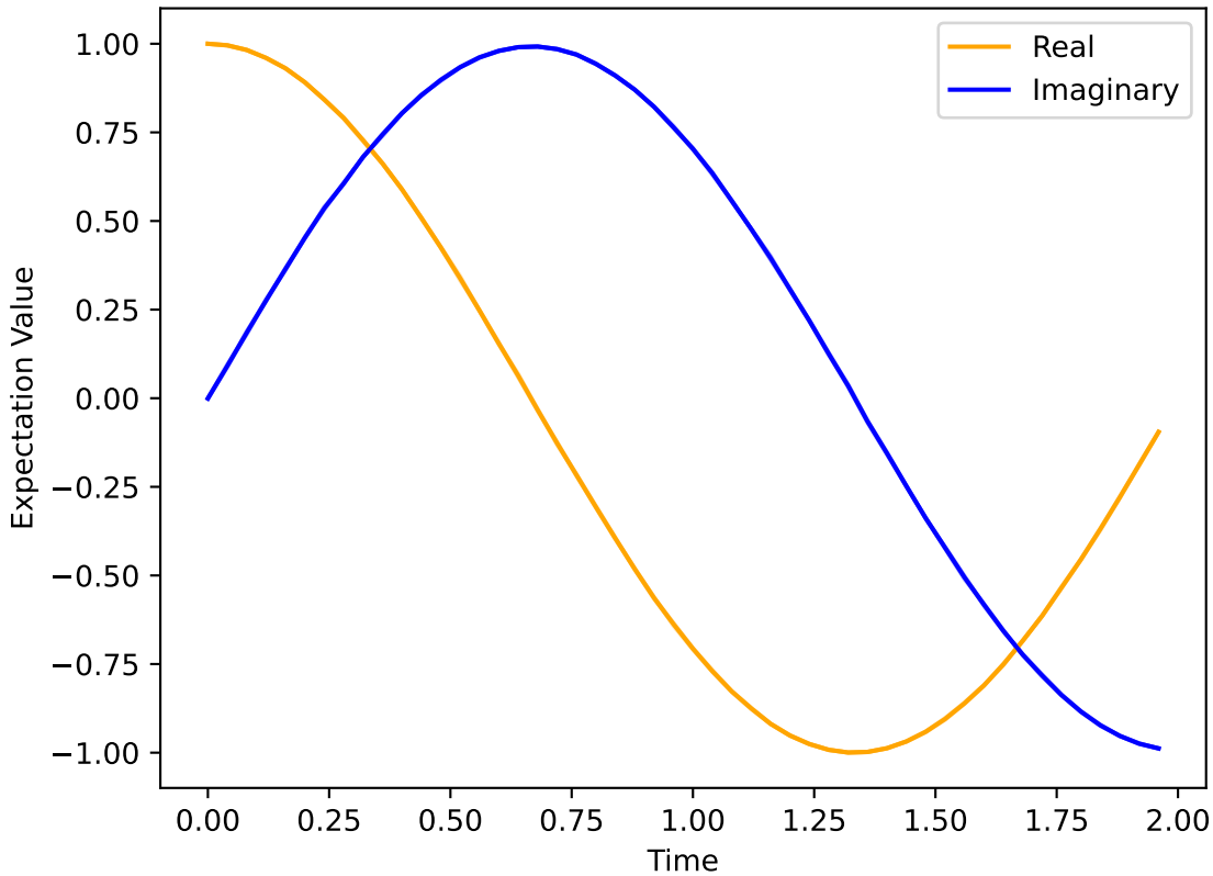
Expectation Value with Dt=0.04
