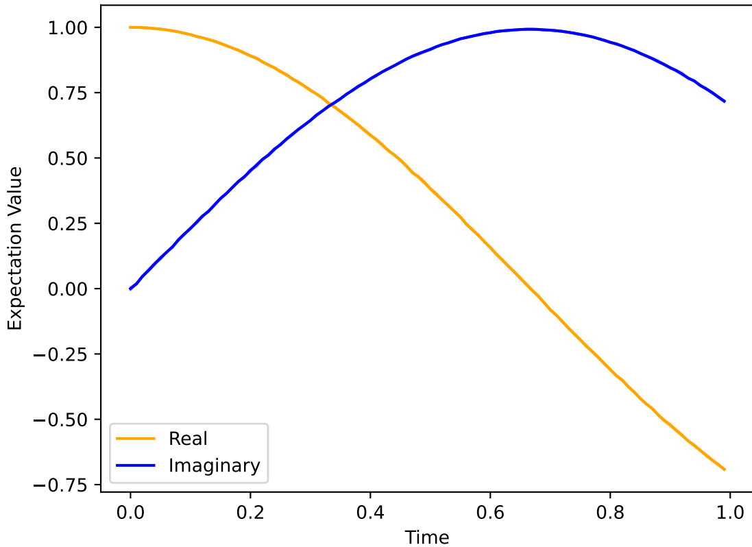
Expectation Value with \Delta t=0.01
