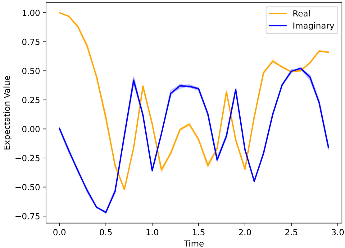
Expectation Value with Dt=0.1
