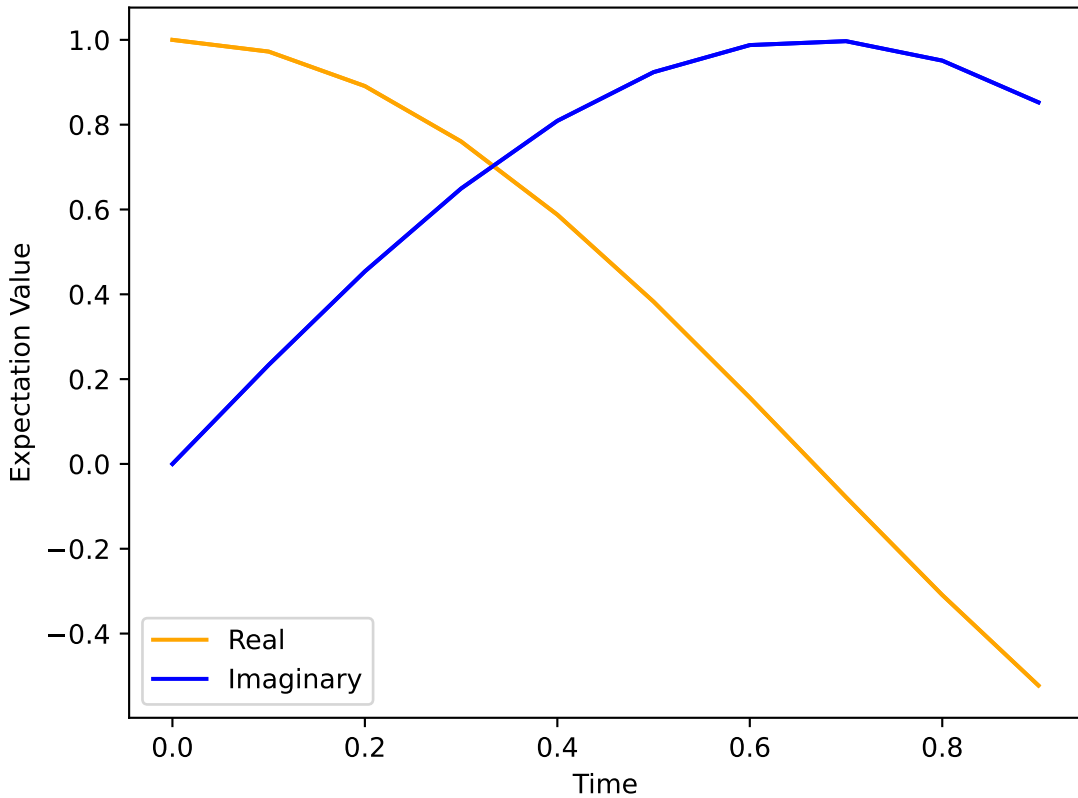
Expectation Value with Dt=0.1
