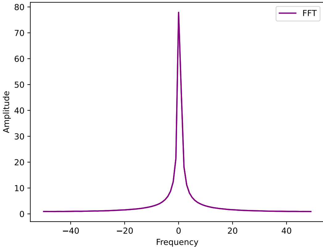
Fourier Transform of Expectation Value with \Delta t=0.01
