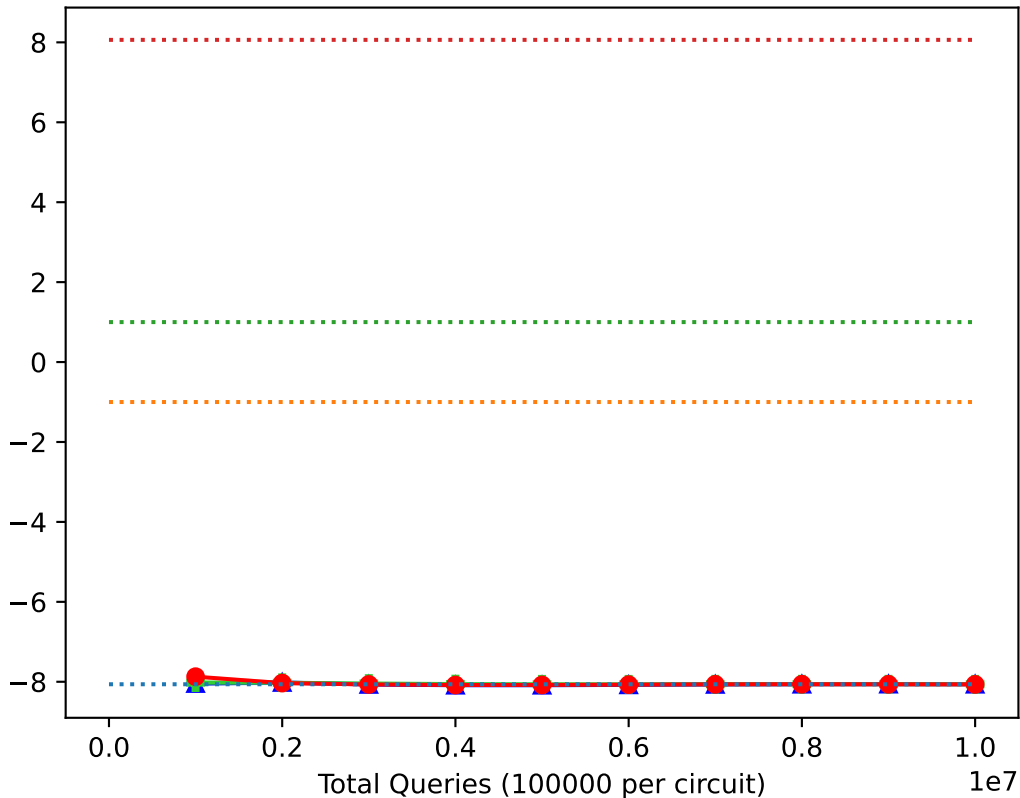
Convergence in Energy for TFI
