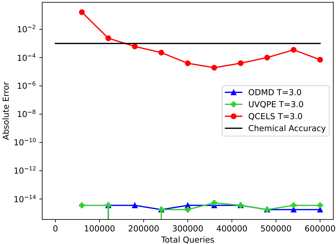
Convergence Absolute Error in Energy for TFI
