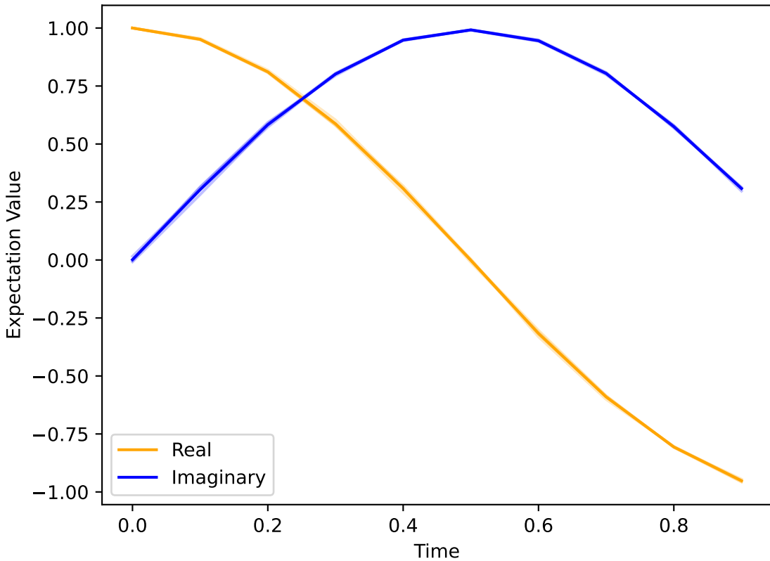
Expectation Value with \Delta t=0.1
