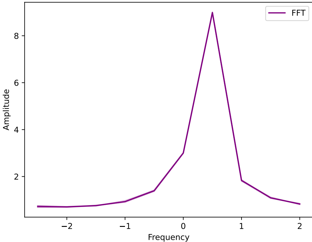
Fourier Transform of Expectation Value with \Delta t=0.2
