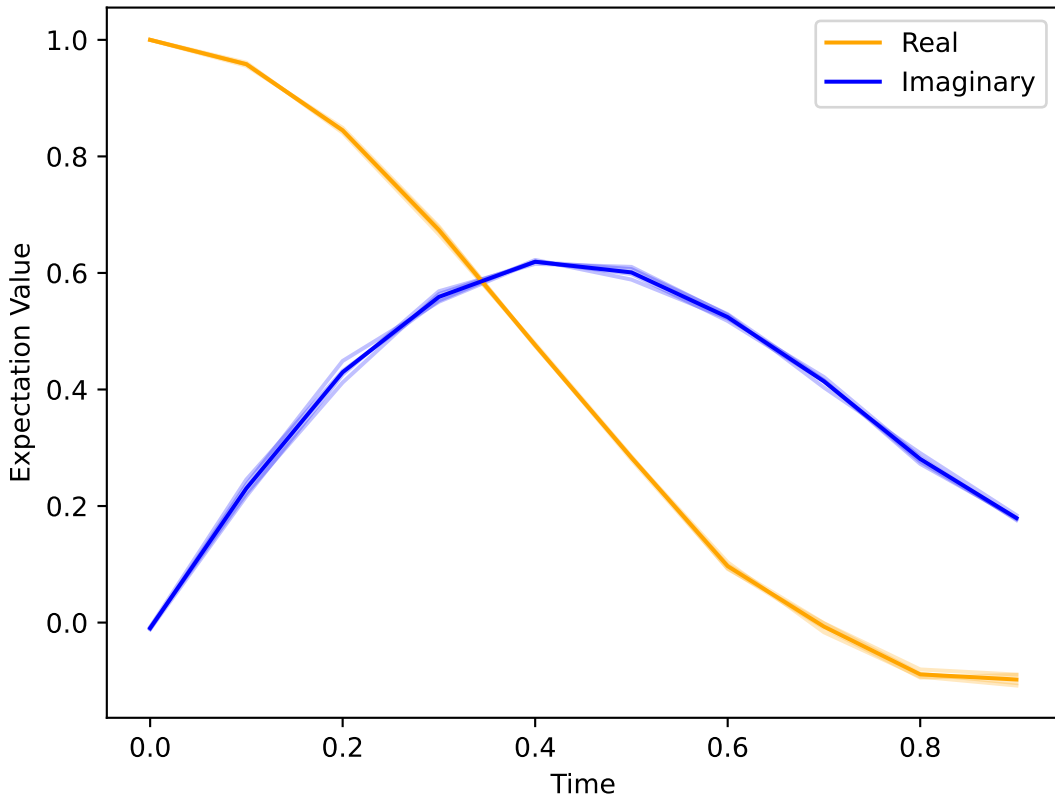
Expectation Value with Dt=0.1
