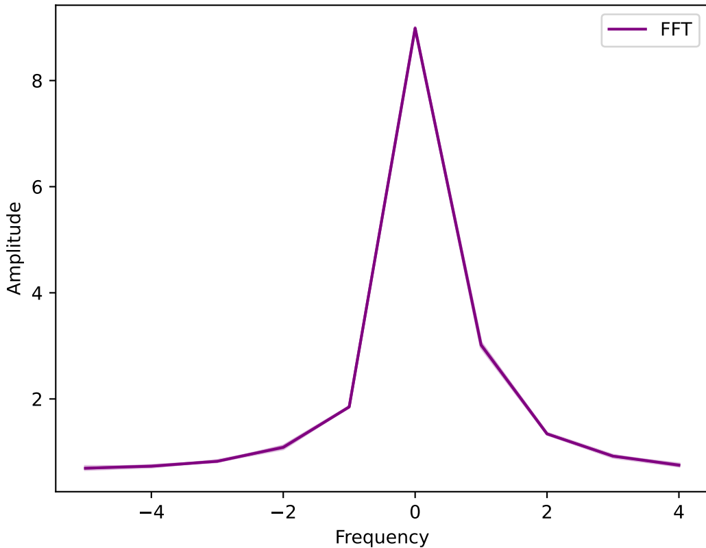
Fourier Transform of Expectation Value with \Delta t=0.1
