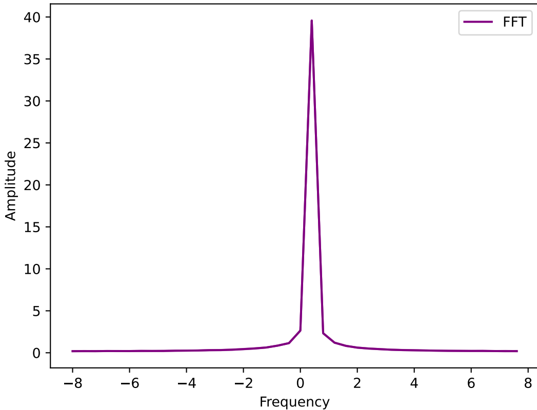
Fourier Transform of Expectation Value with \Delta t=0.0625
