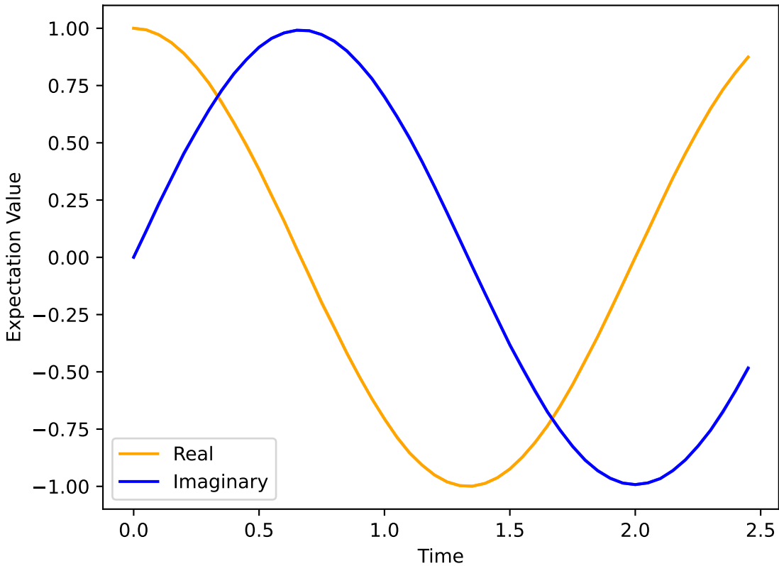
Expectation Value with \Delta t=0.05
