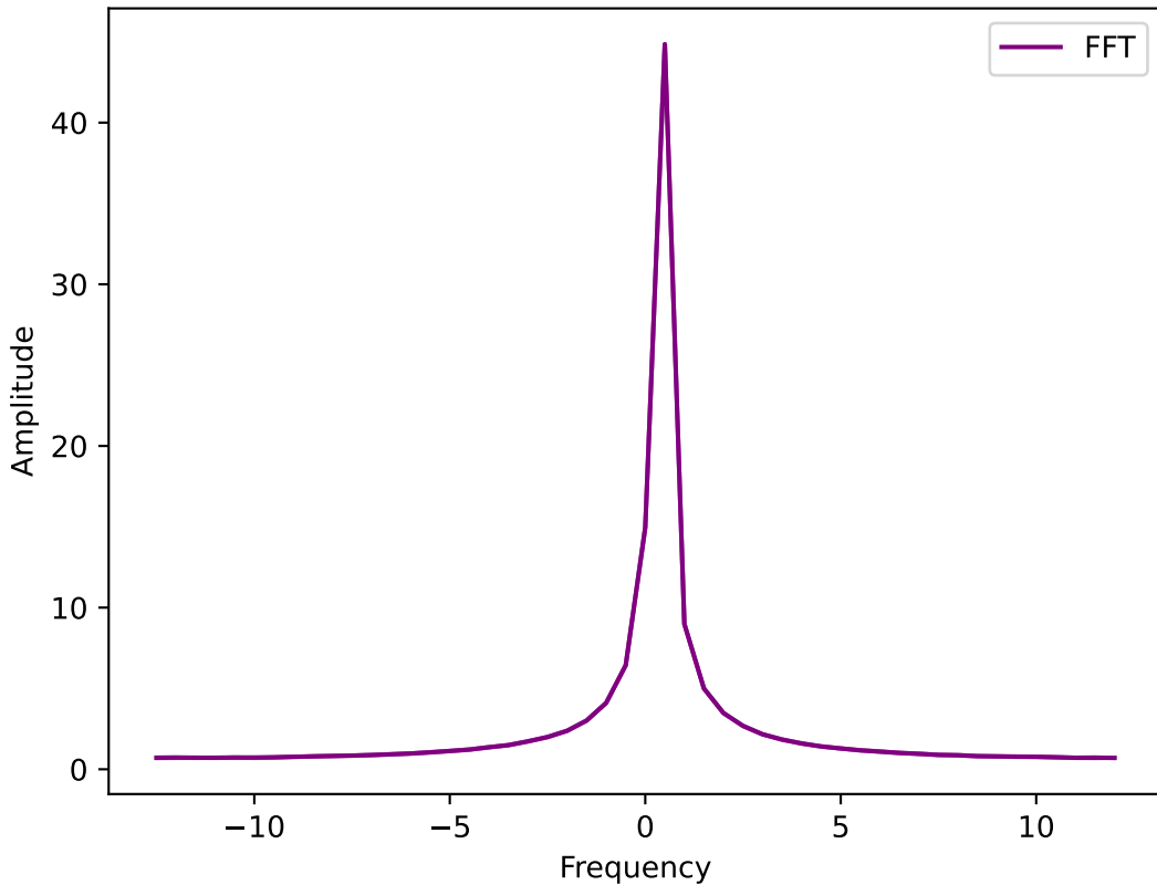
Fourier Transform of Expectation Value with \Delta t=0.04
