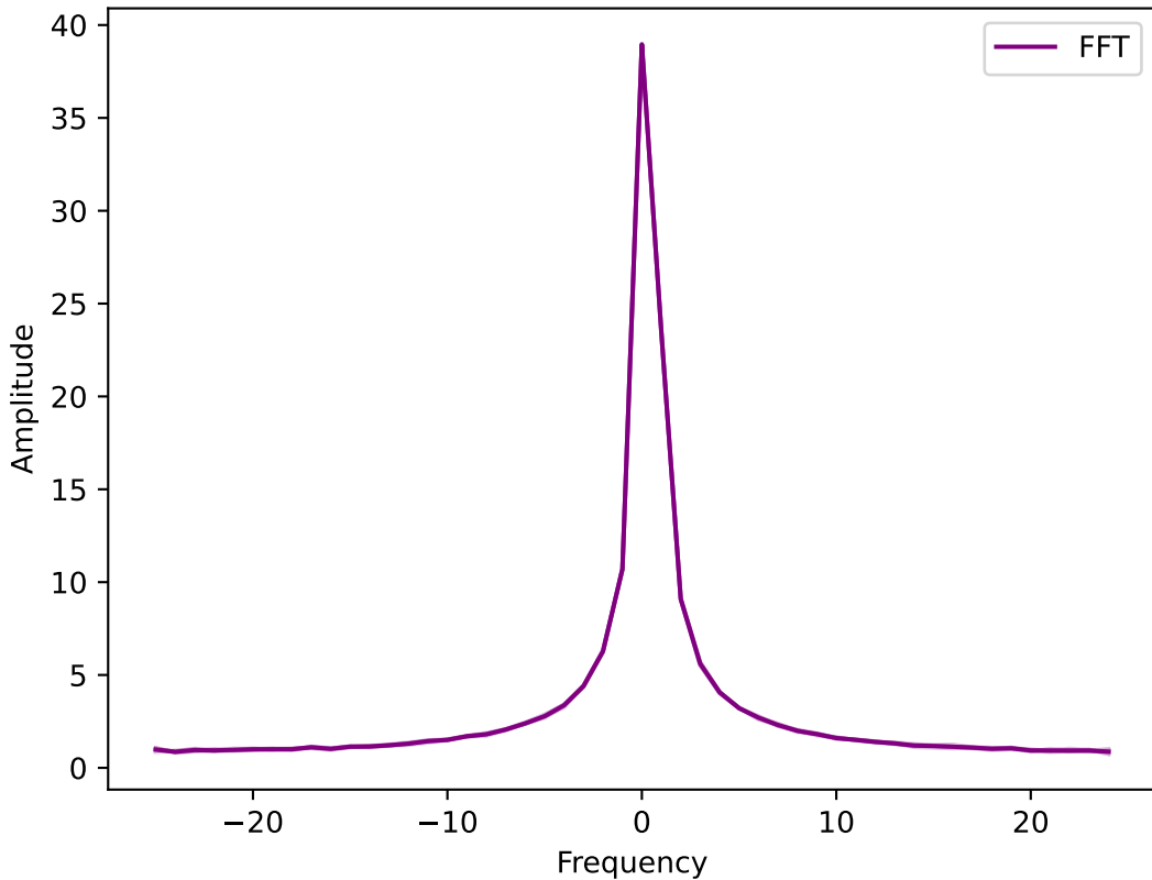
Fourier Transform of Expectation Value with \Delta t=0.02
