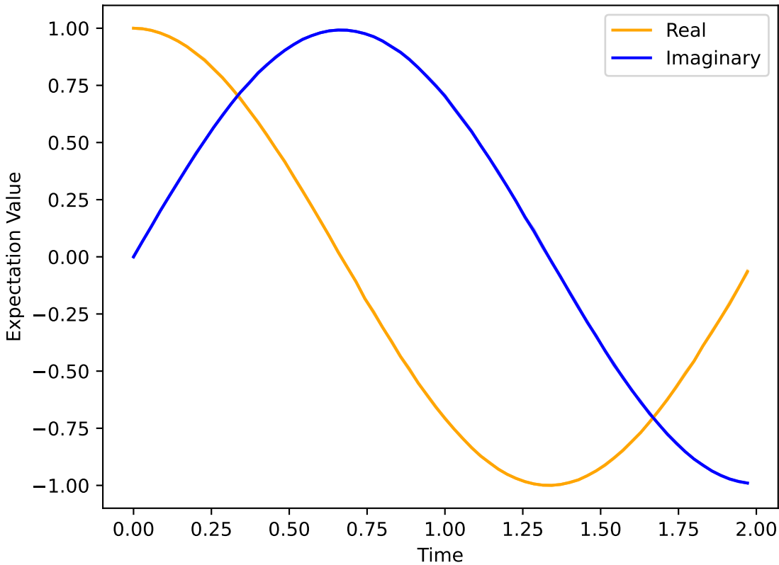
Expectation Value with \Delta t=0.02857142857142857
