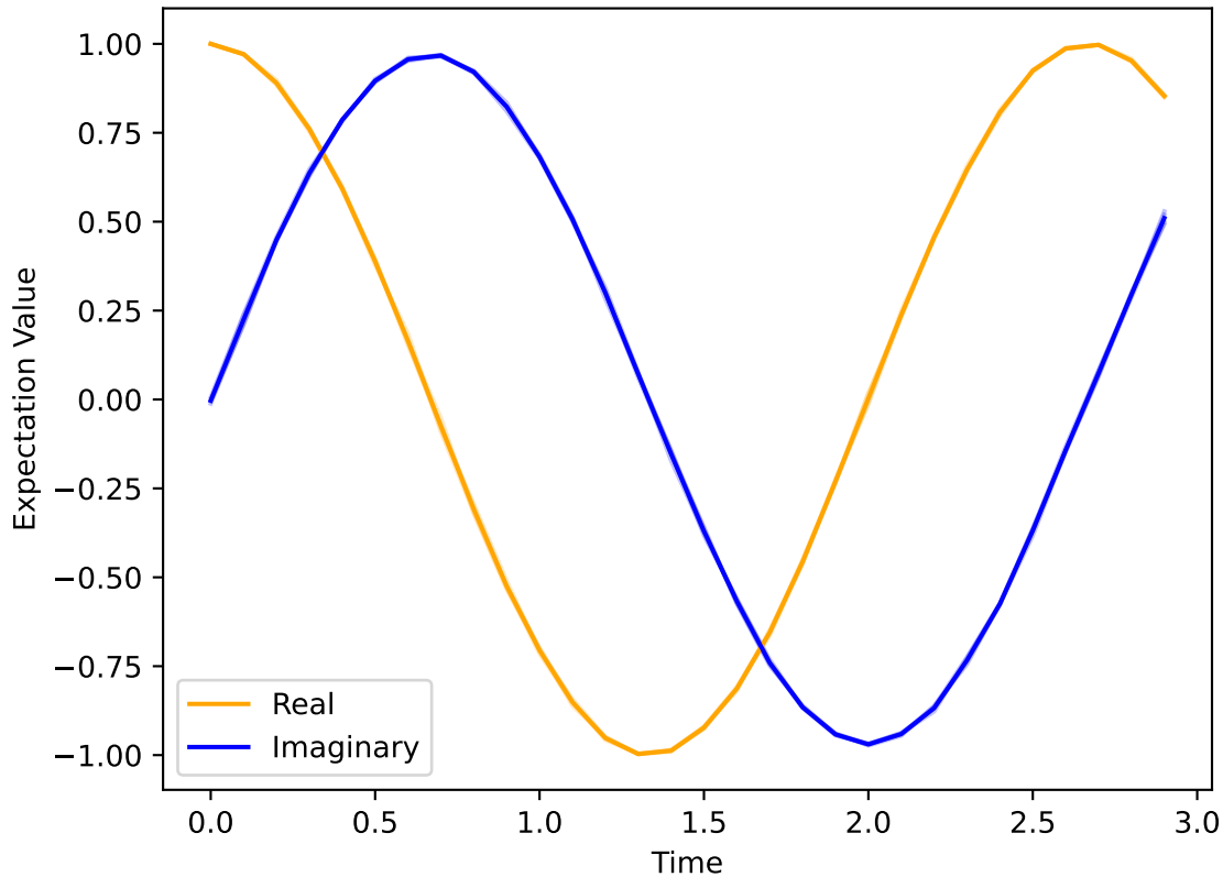
Expectation Value with \Delta t=0.1
