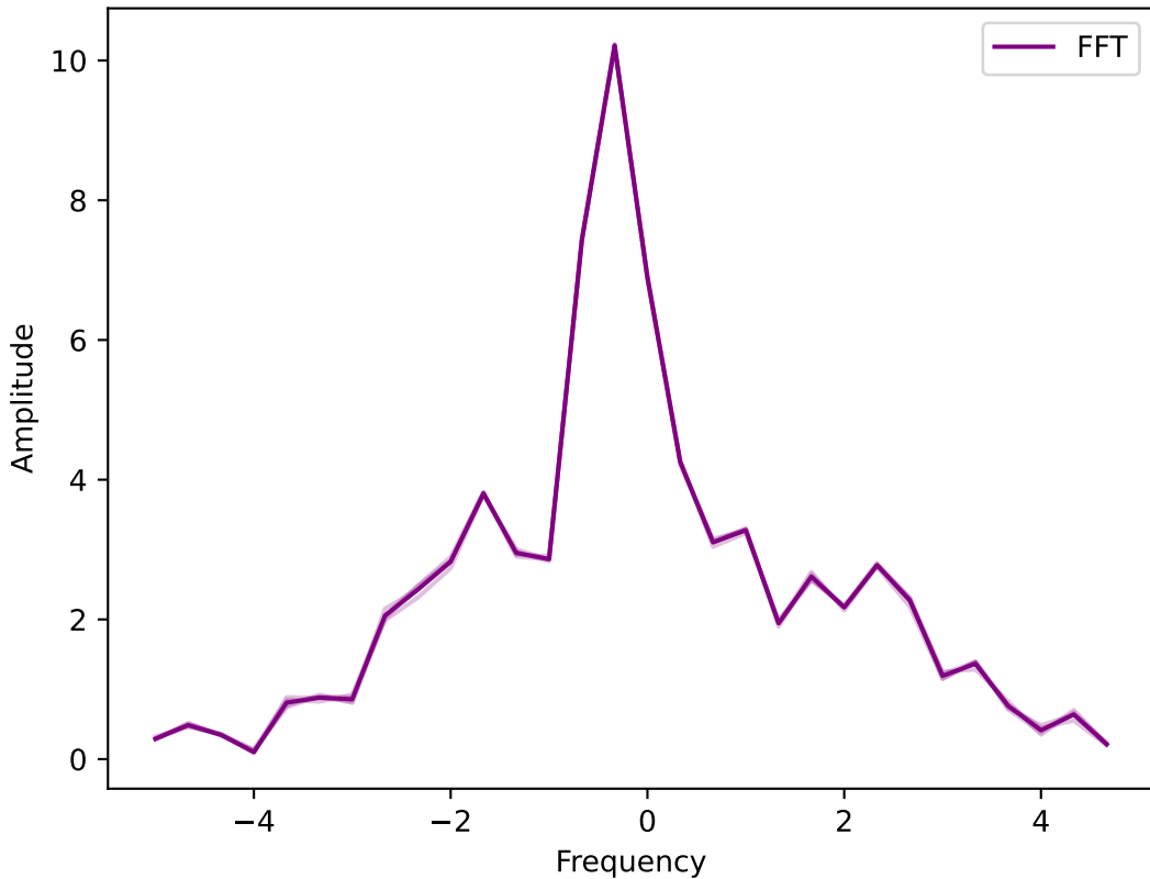
Fourier Transform of Expectation Value with Dt=0.1
