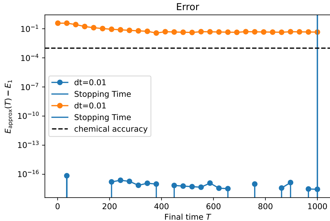
Hubbard (1 sites, T=1 , V=1.5 | targeted particle number 1.0)
