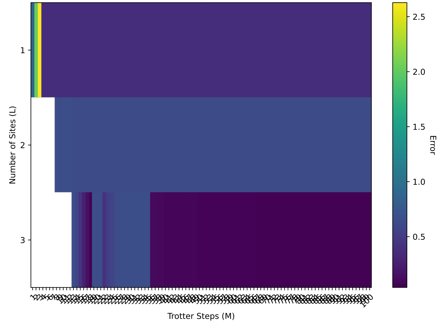
Hubbard (3 sites, T=1 , V=1.5 | targeted particle number 3.0)
