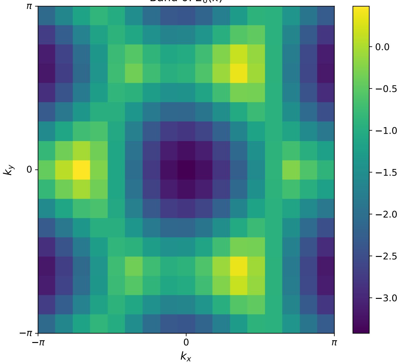
Band 0: E_0(k)
