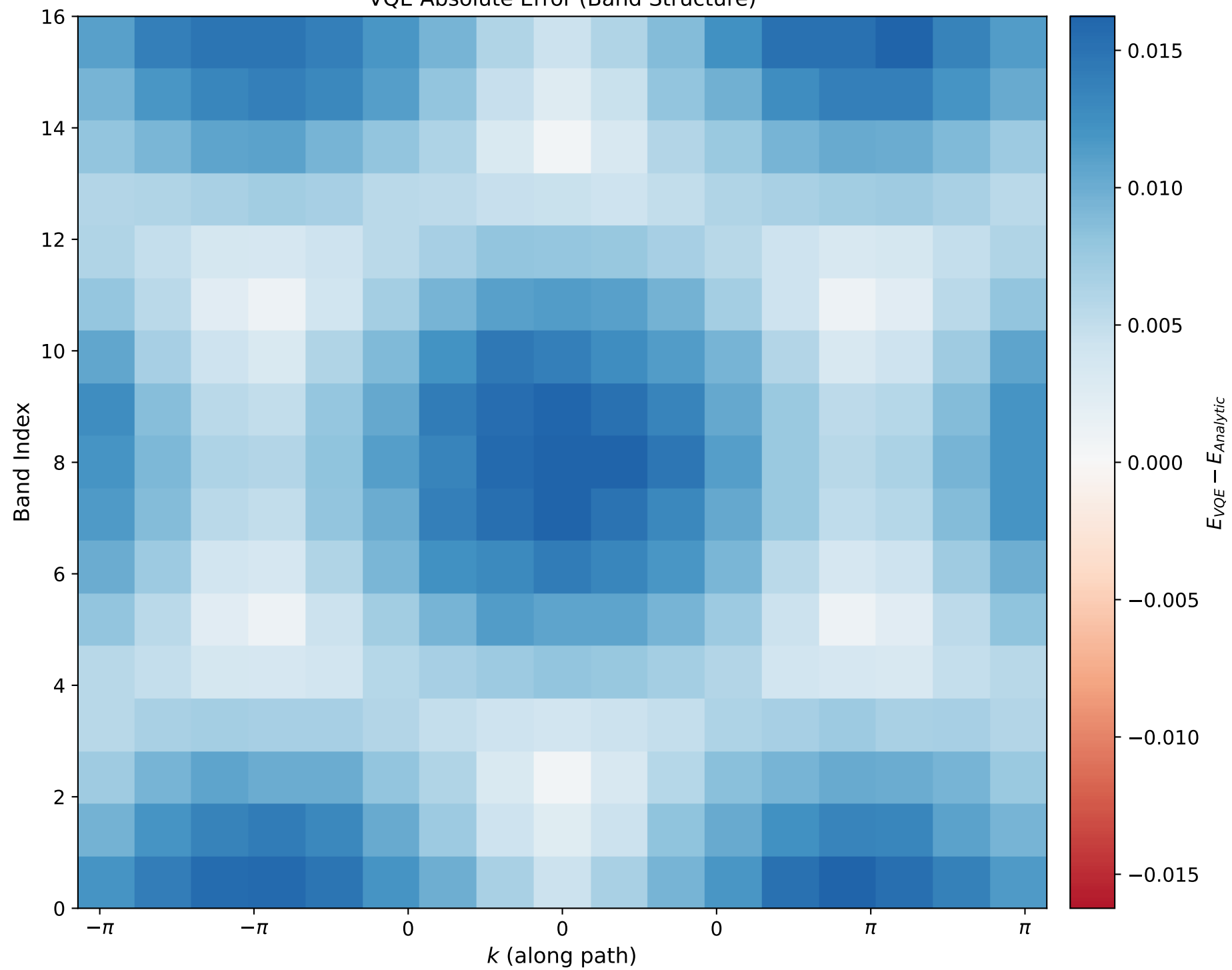
VQE Absolute Error (Band Structure)
