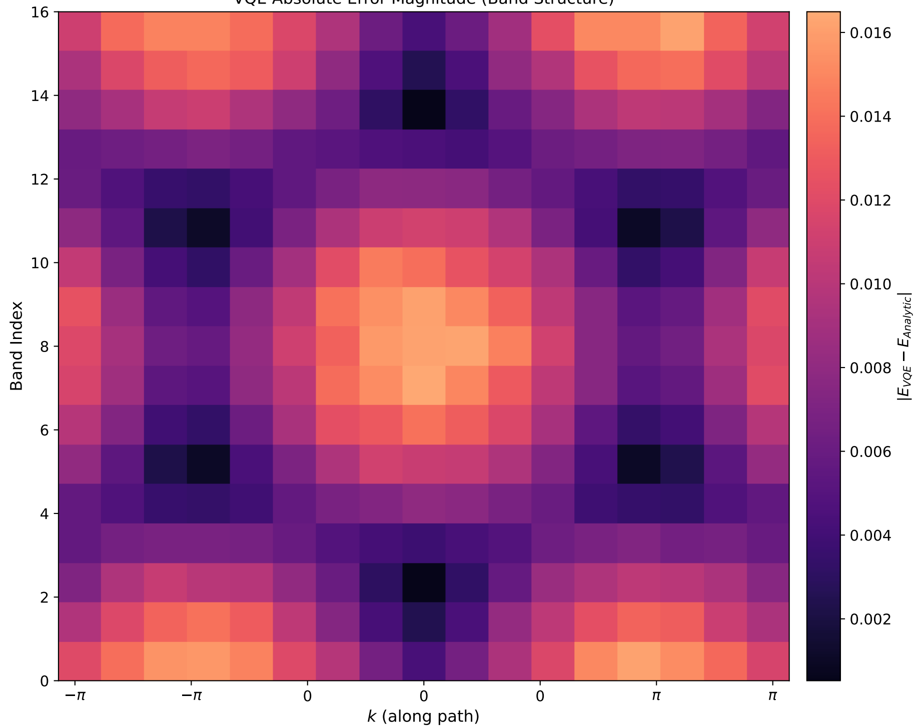
VQE Absolute Error Magnitude (Band Structure)
