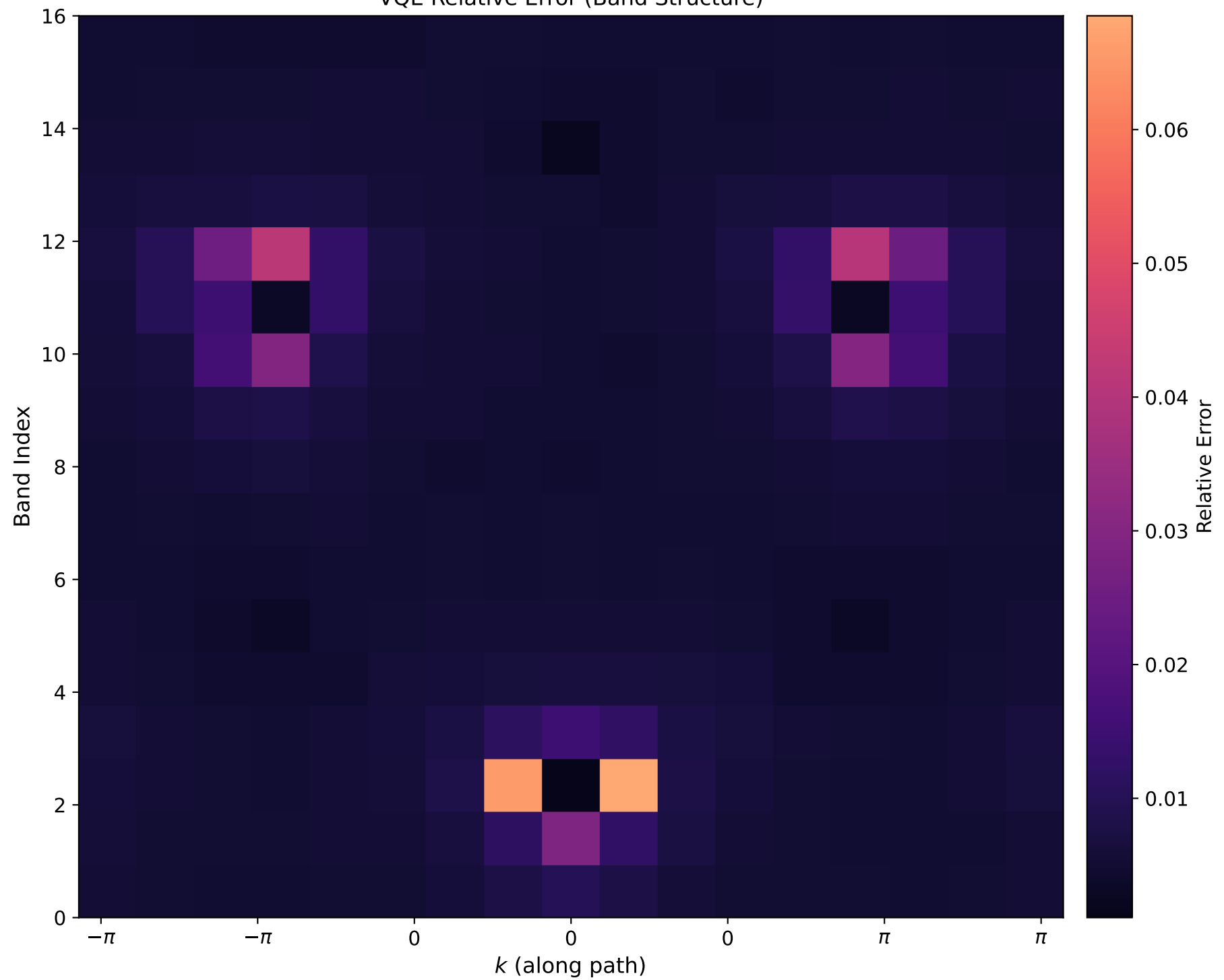
VQE Relative Error (Band Structure)
