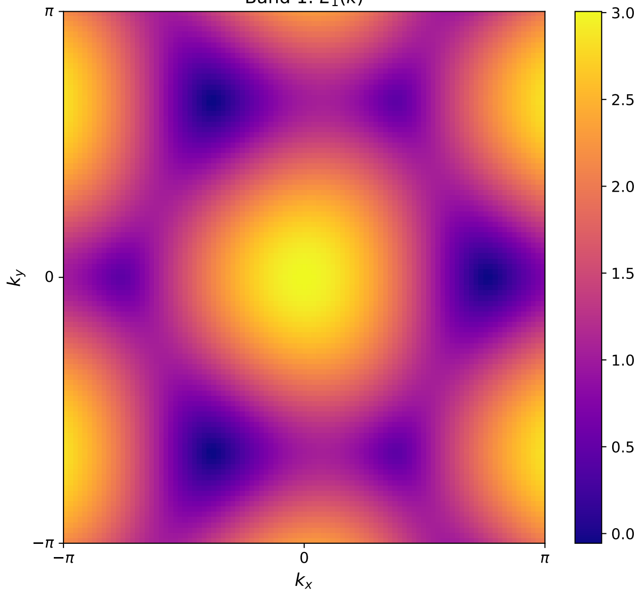
Band 1: E_1(k)
