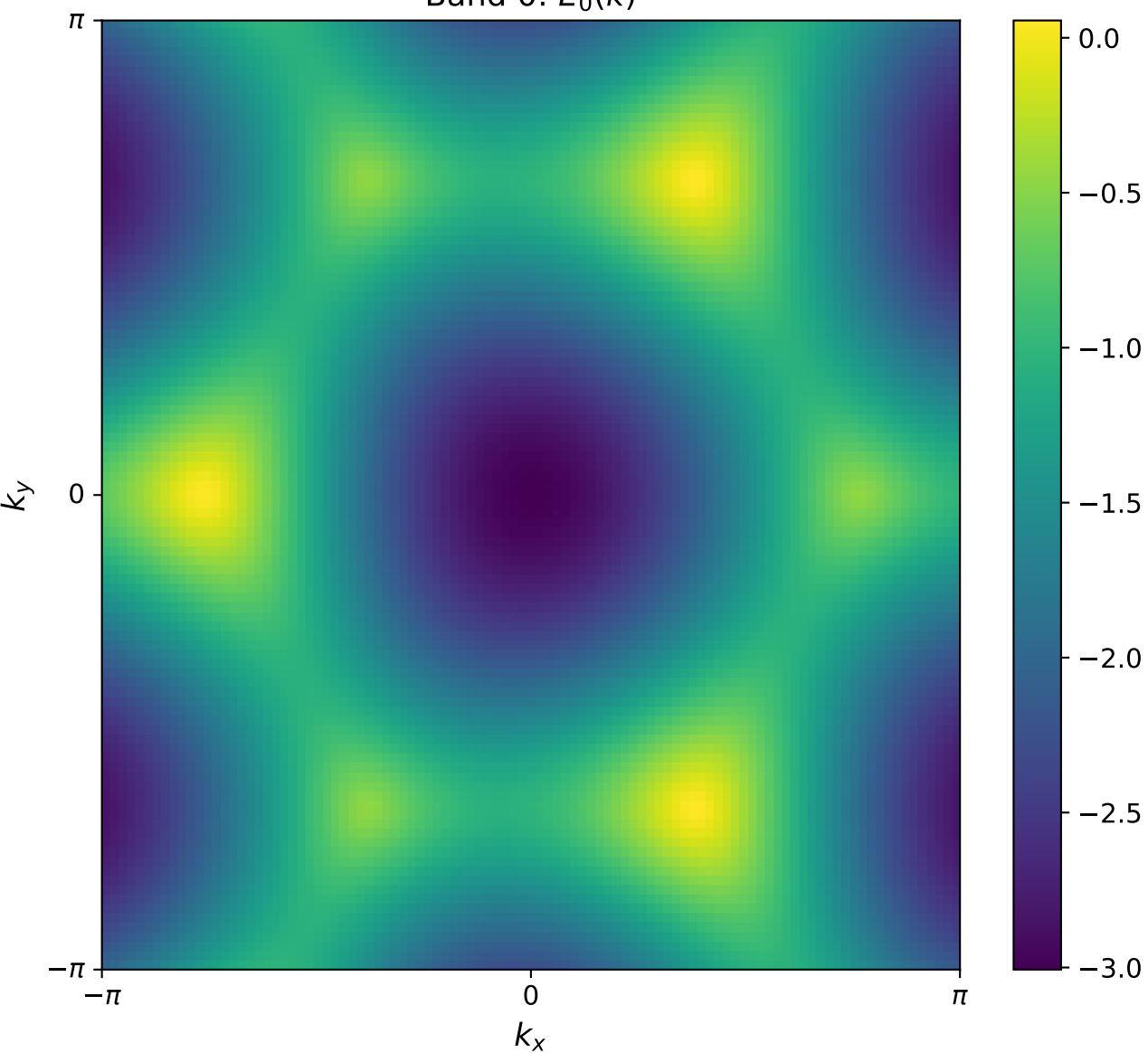
Band 0: E_0(k)
