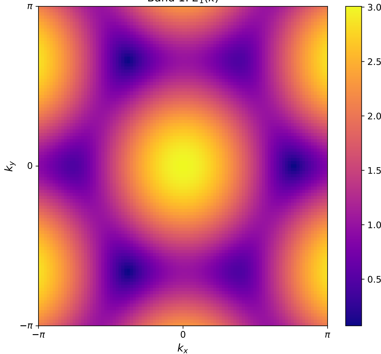
Band 1: E_1(k)
