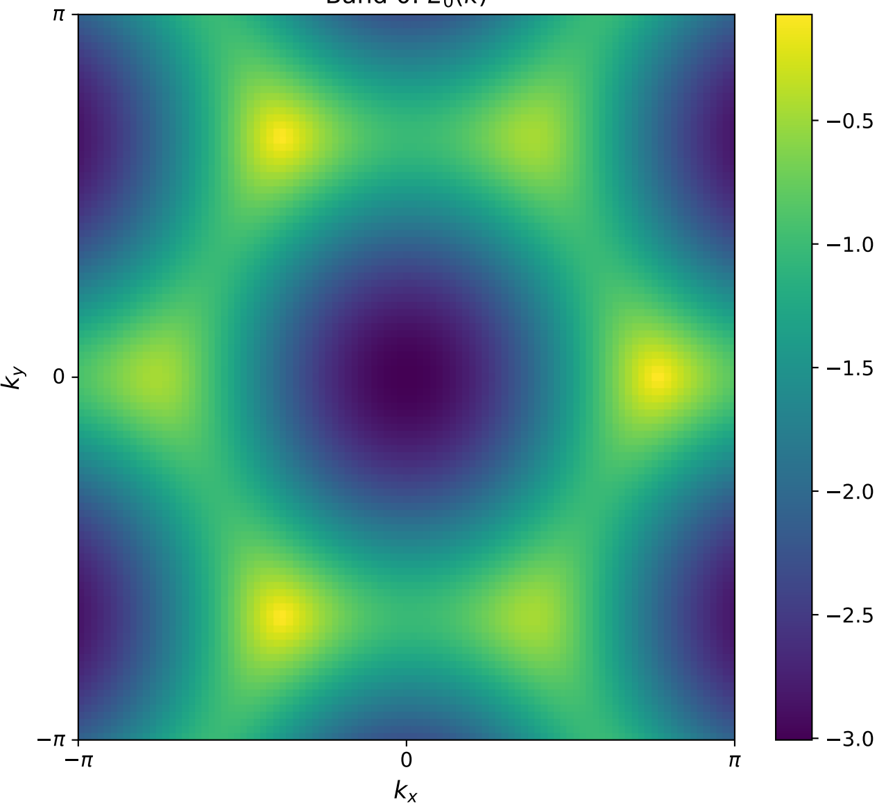
Band 0: E_0(k)
