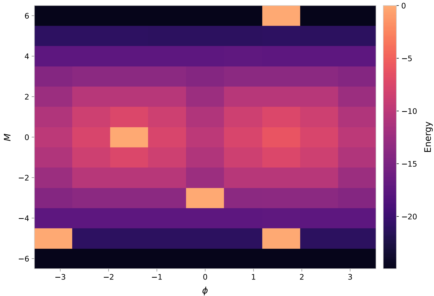
DMRG
