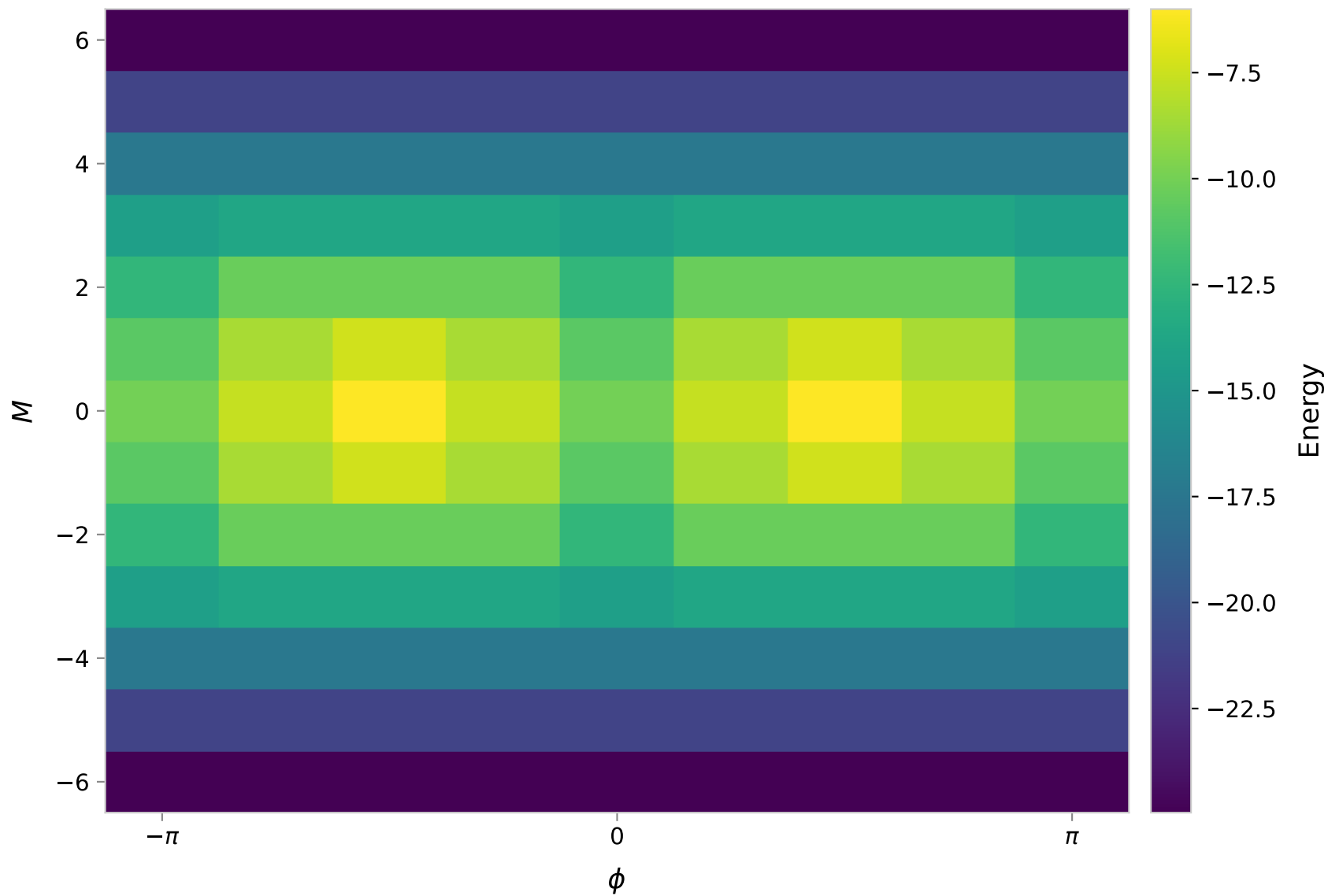
Ground State Energy (ANALYTIC)
