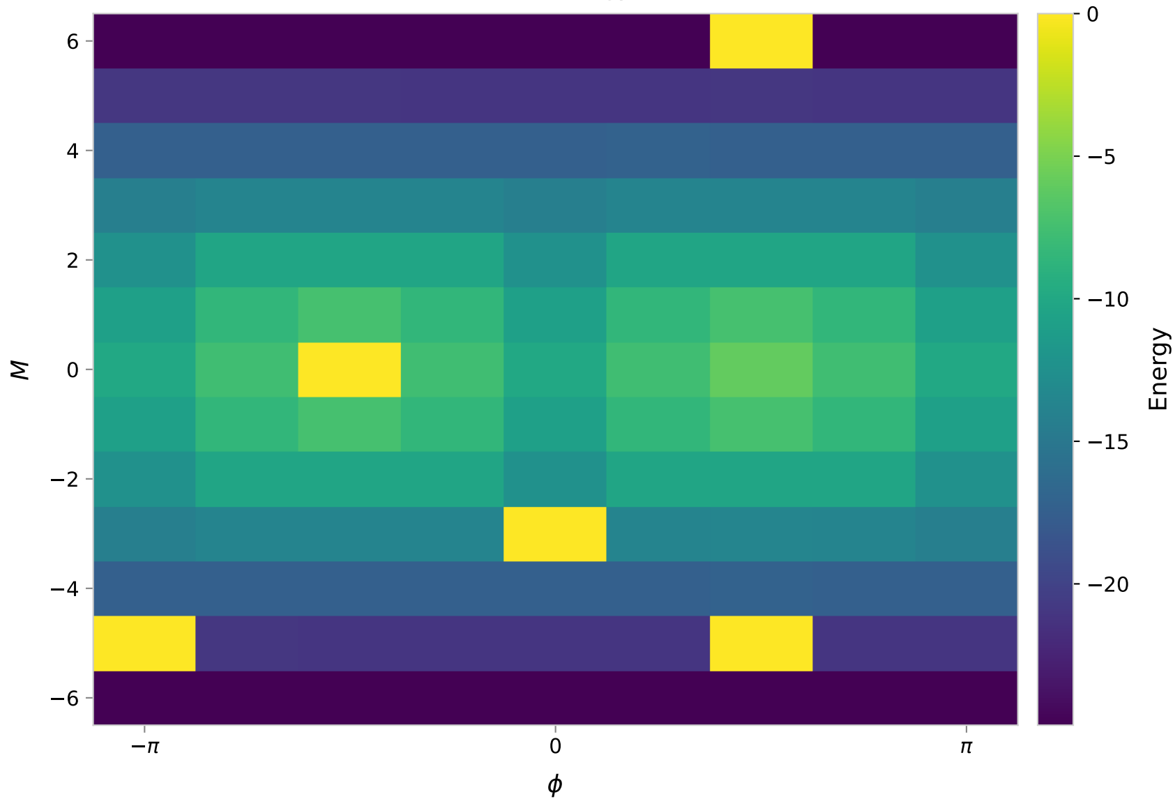
Ground State Energy (DMRG)
