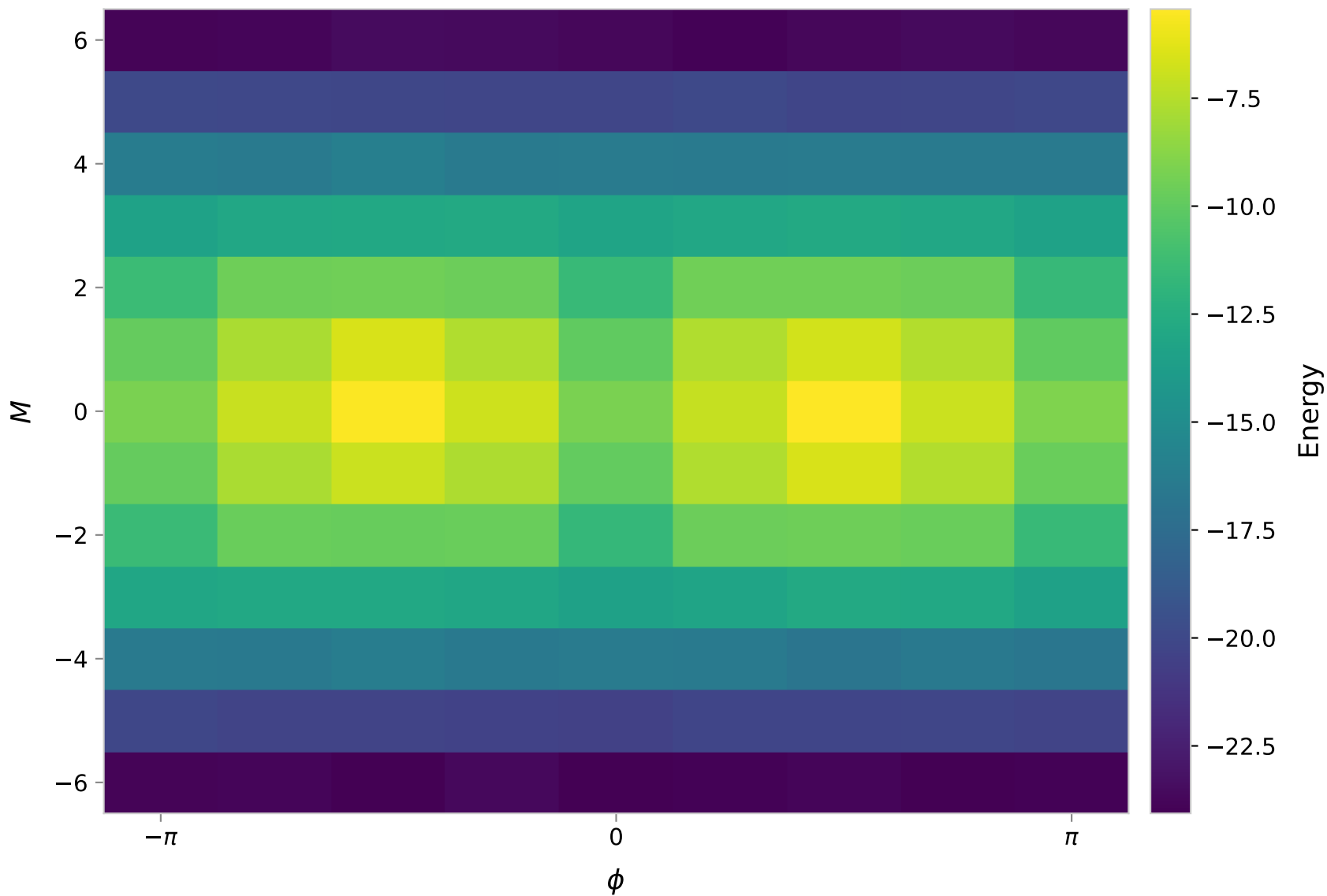
Ground State Energy (VQE)
