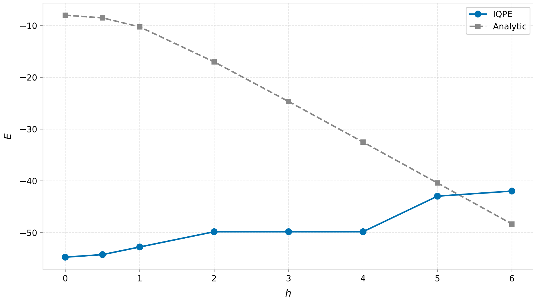
TFIM 1D ( L_x=8 , PBC) - Ground State Energy ( t=0.1 )
