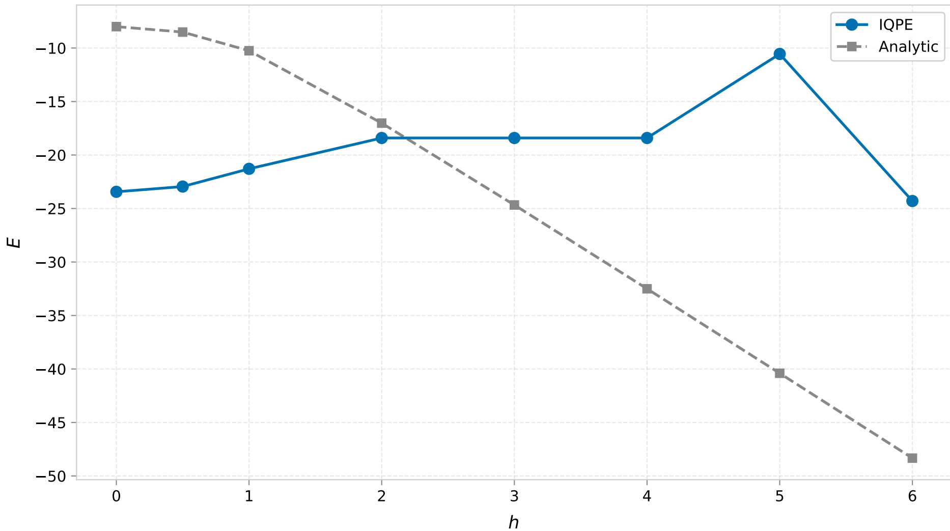
TFIM 1D ( L_x=8 , PBC) - Ground State Energy ( t=0.2 )
