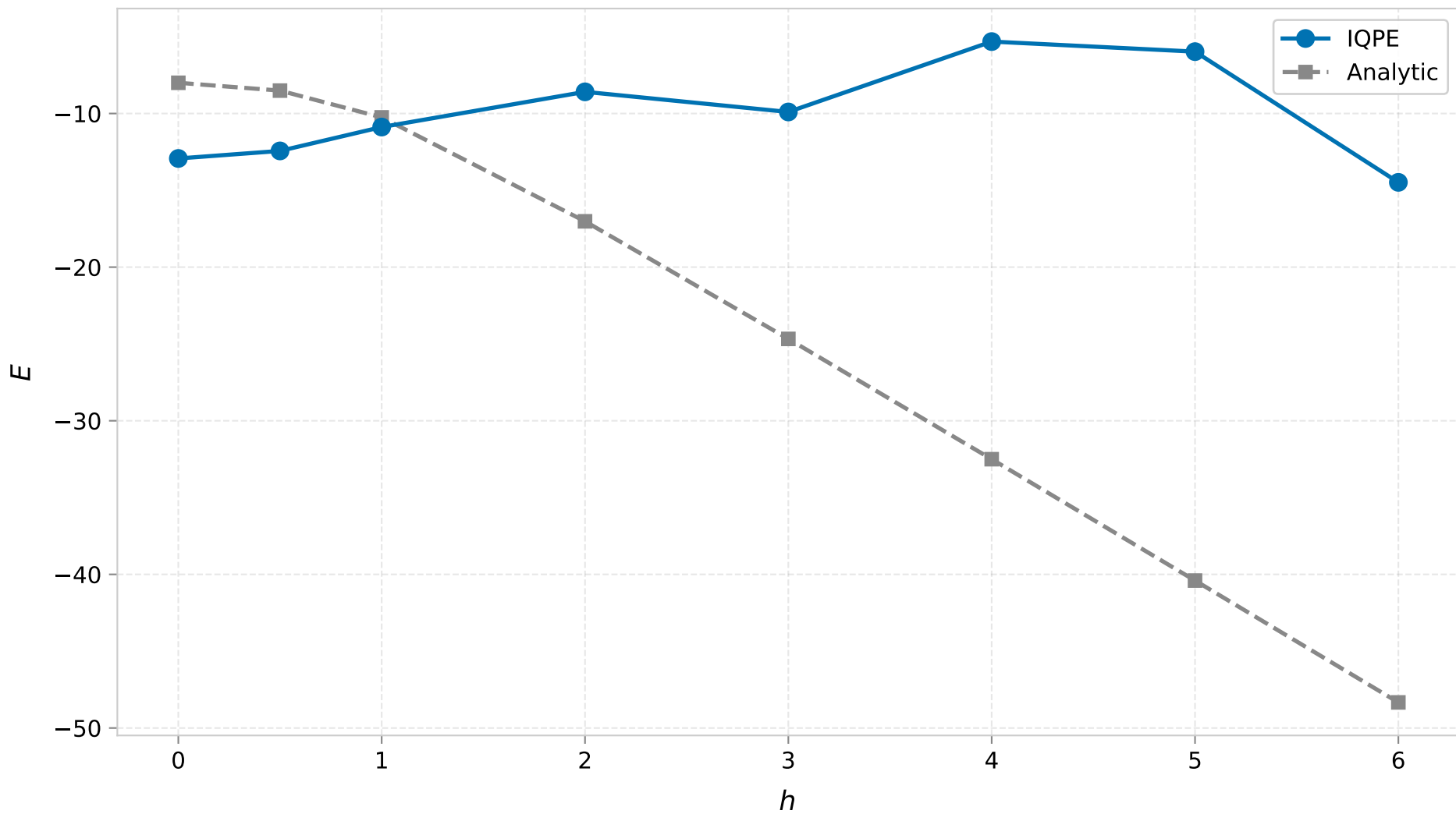
TFIM 1D ( L_x=8 , PBC) - Ground State Energy ( t=0.3 )
