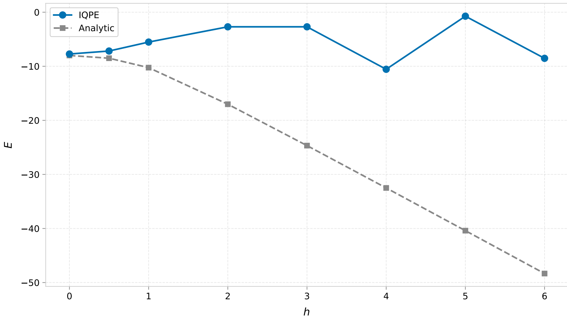
TFIM 1D ( L_x=8 , PBC) - Ground State Energy ( t=0.4 )
