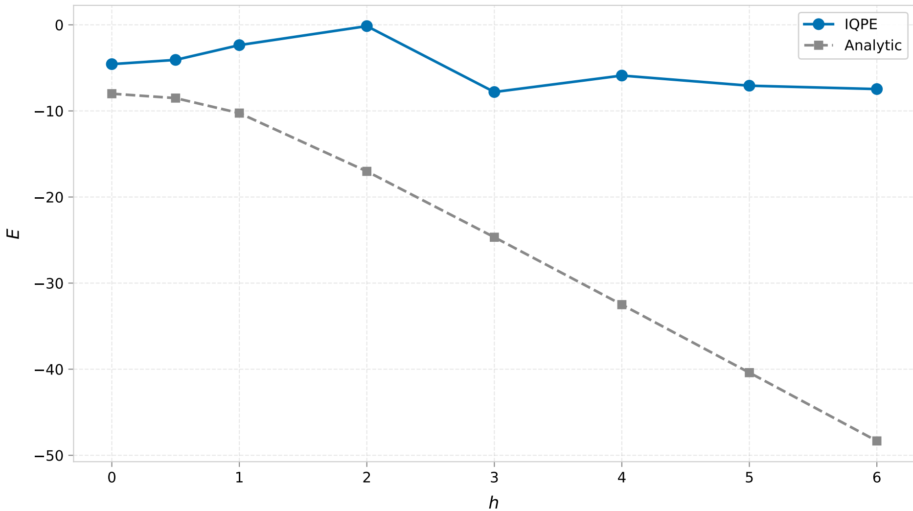
TFIM 1D ( L_x=8 , PBC) - Ground State Energy ( t=0.5 )
