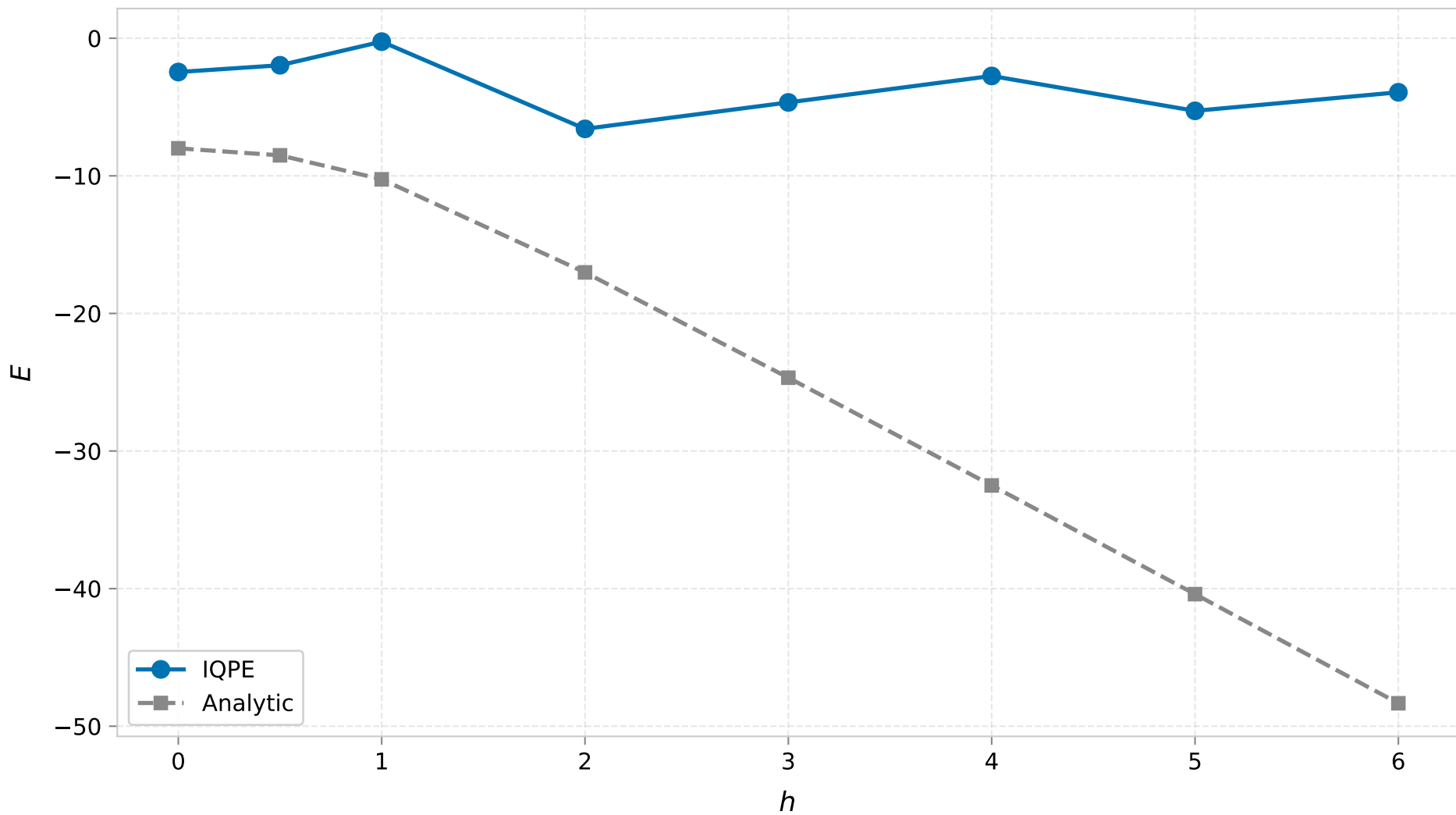
TFIM 1D ( L_x=8 , PBC) - Ground State Energy ( t=0.6 )
