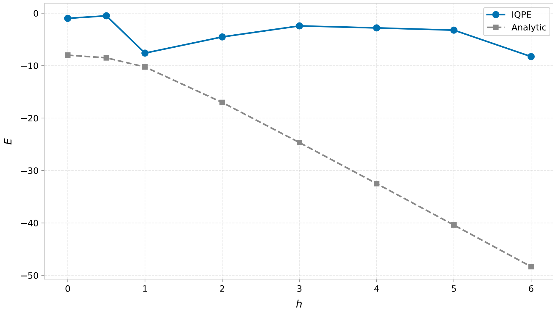
TFIM 1D ( L_x=8 , PBC) - Ground State Energy ( t=0.7 )
