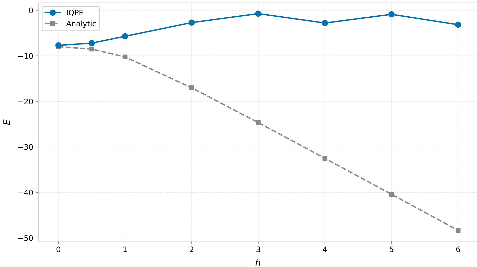
TFIM 1D ( L_x=8 , PBC) - Ground State Energy ( t=0.8 )
