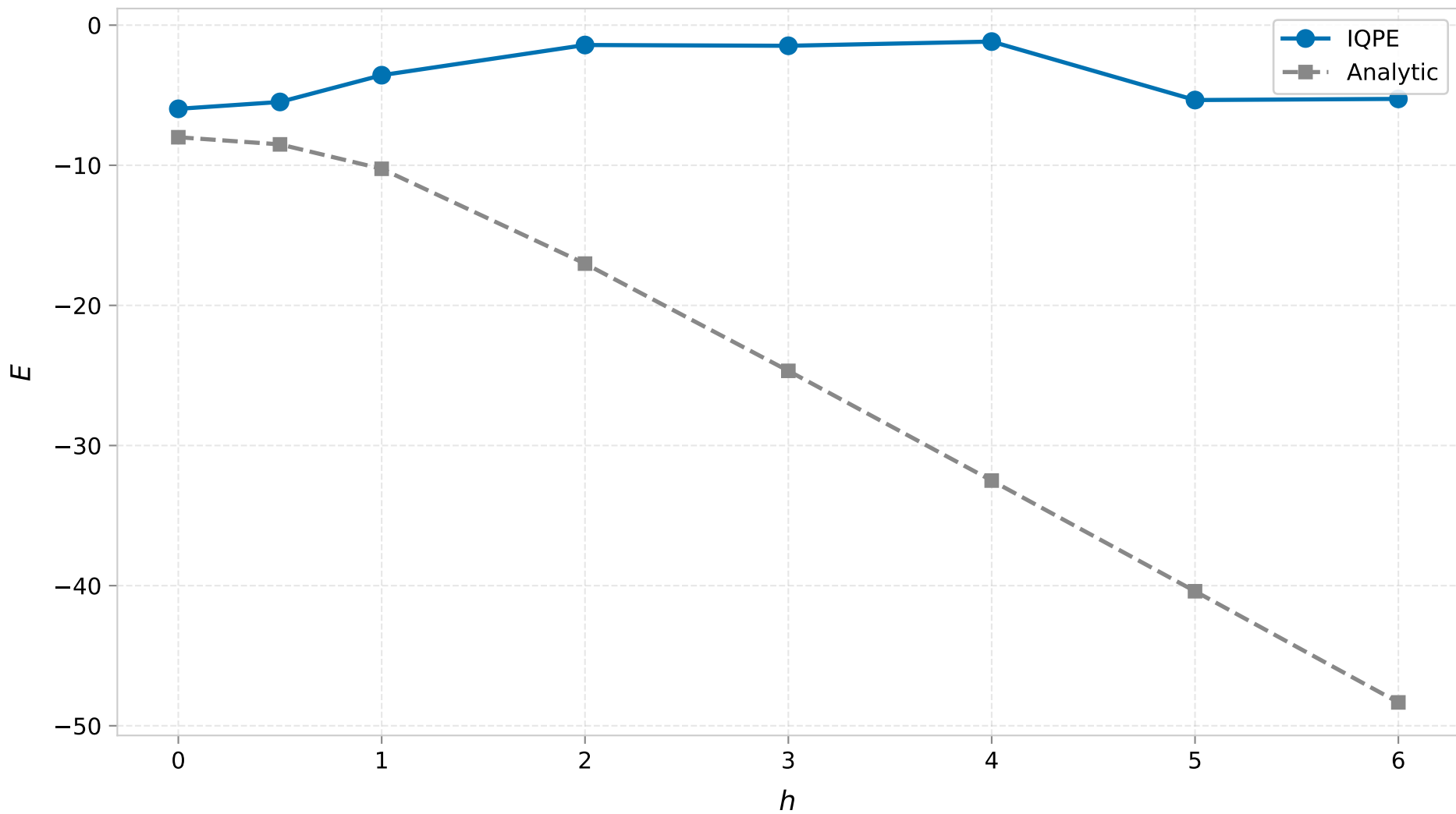
TFIM 1D ( L_x=8 , PBC) - Ground State Energy ( t=0.9 )
