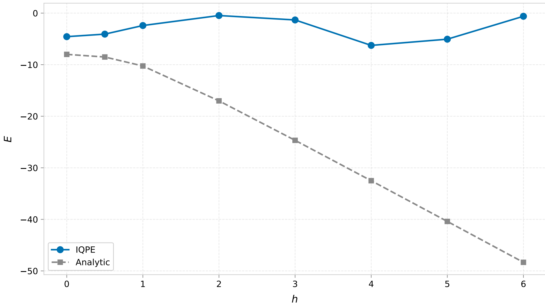
TFIM 1D ( L_x=8 , PBC) - Ground State Energy ( t=1.0 )
