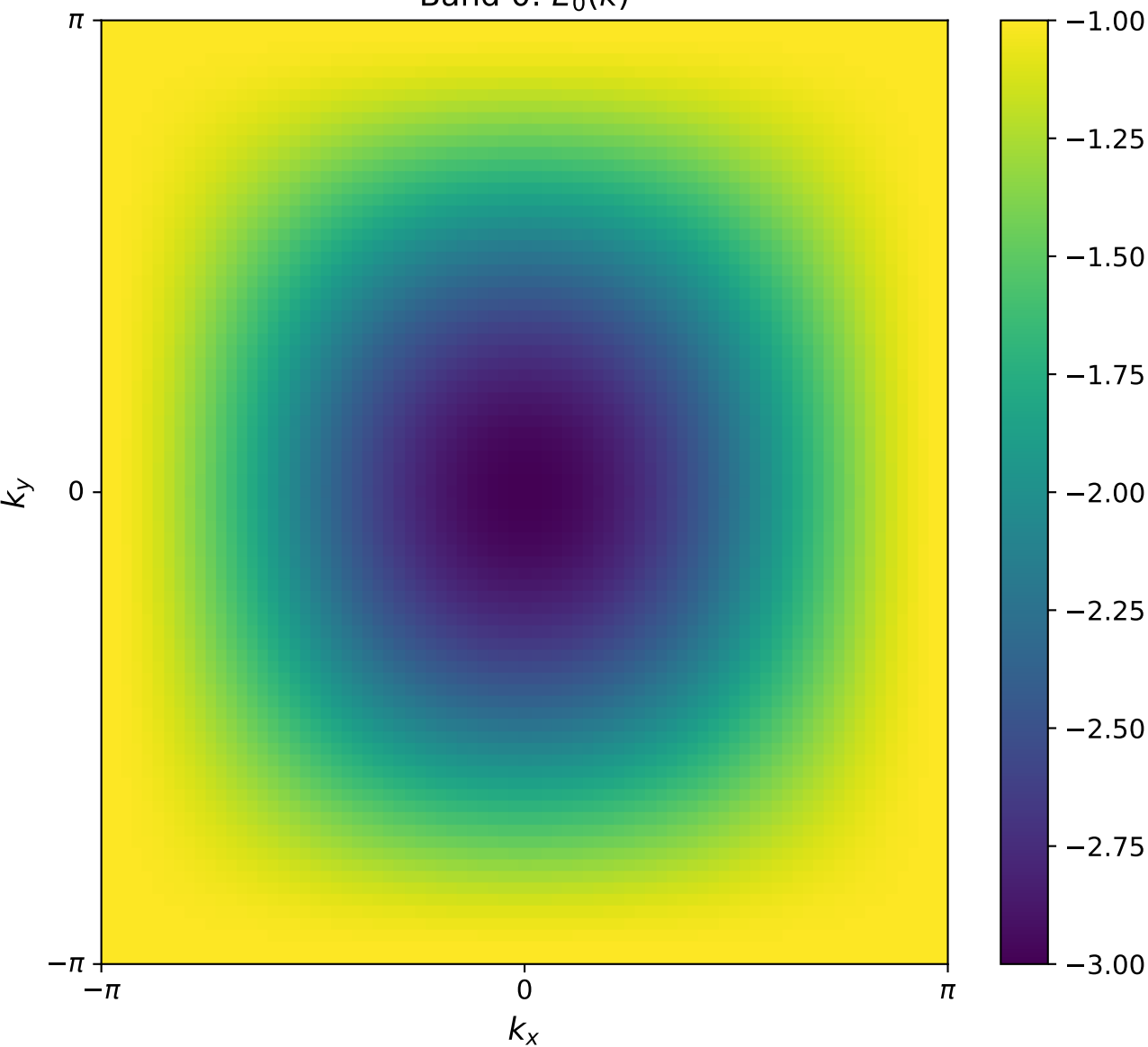
Band 0: E_0(k)
