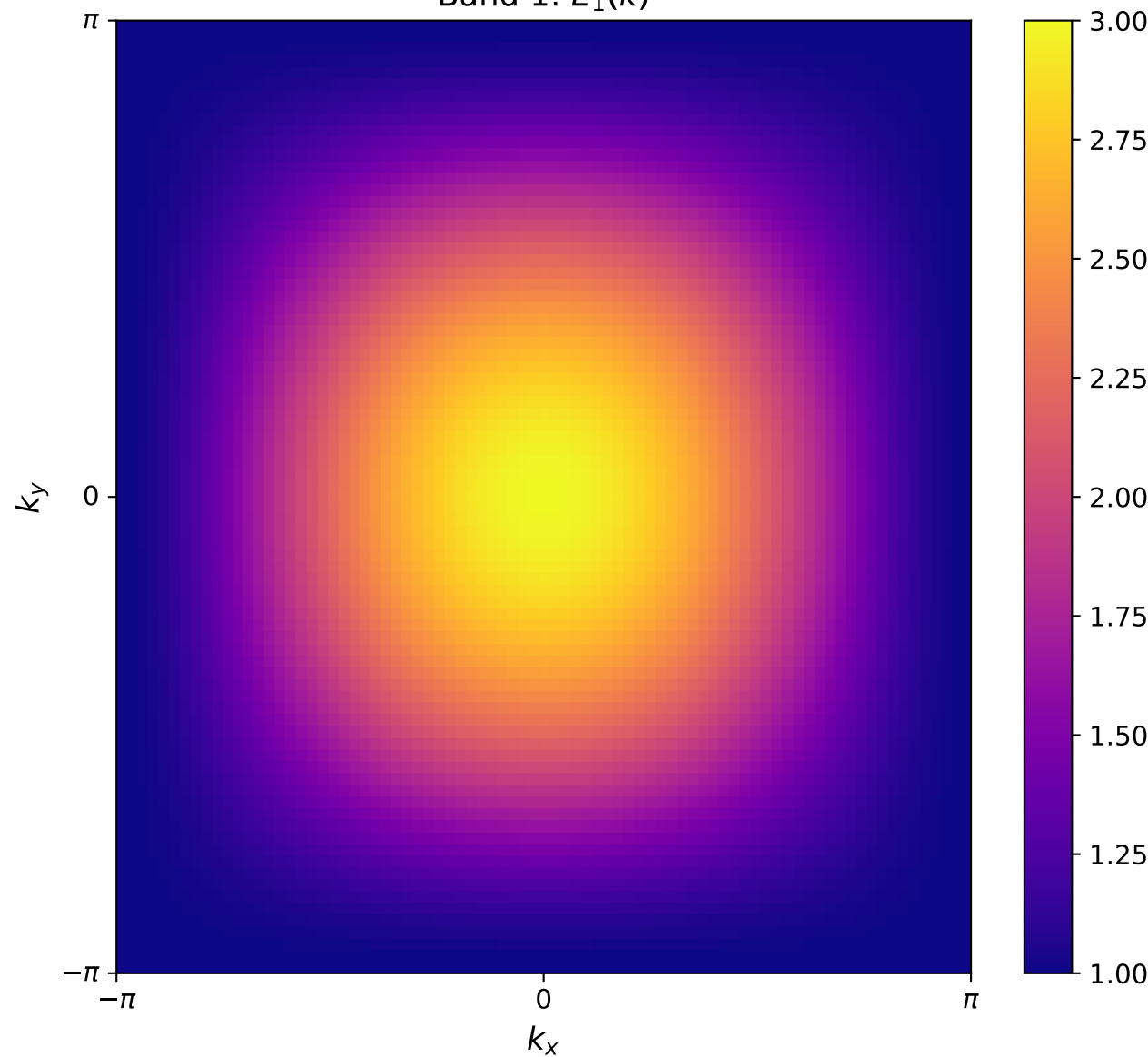
Band 1: E_1(k)
