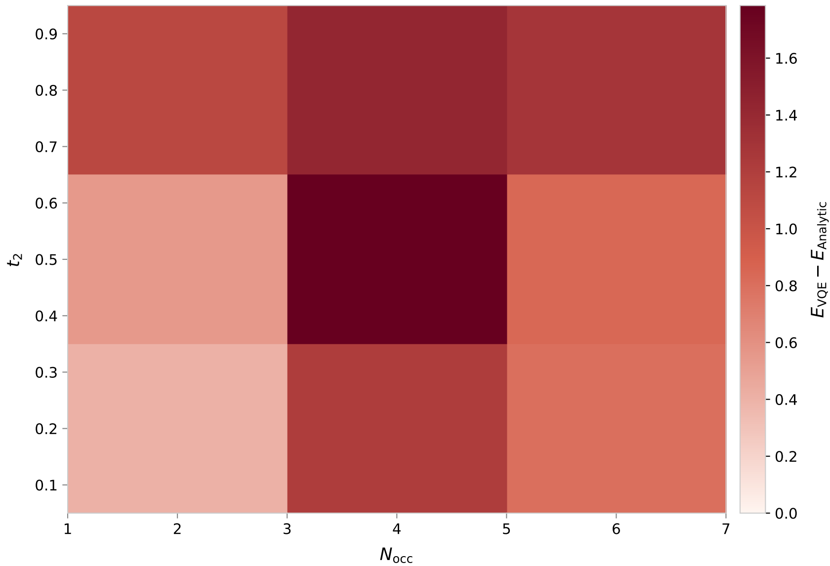
Haldane, 2×2, VQE – Analytic
