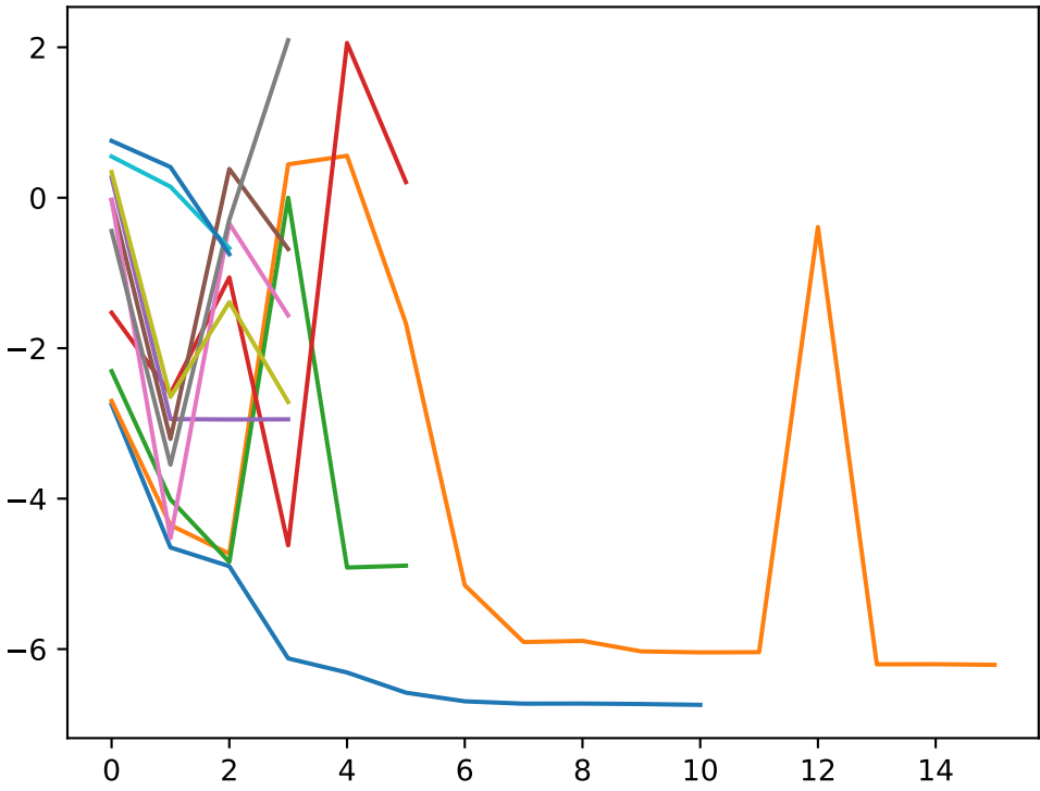
Exact derivative
