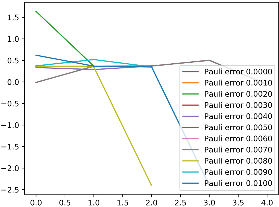
Numerical derivative
