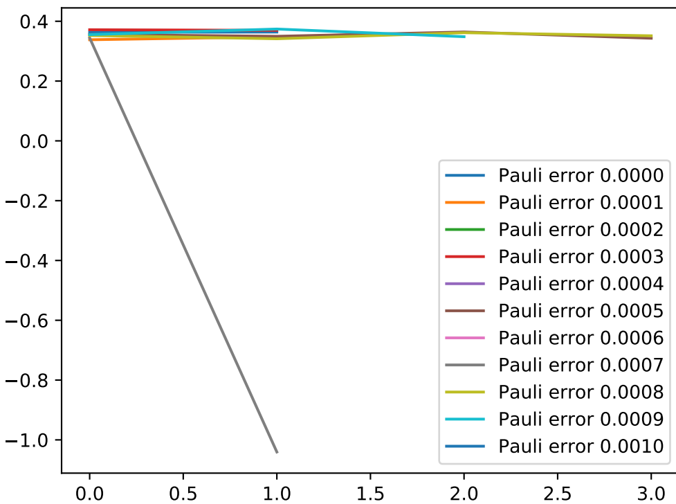
Numerical derivative
