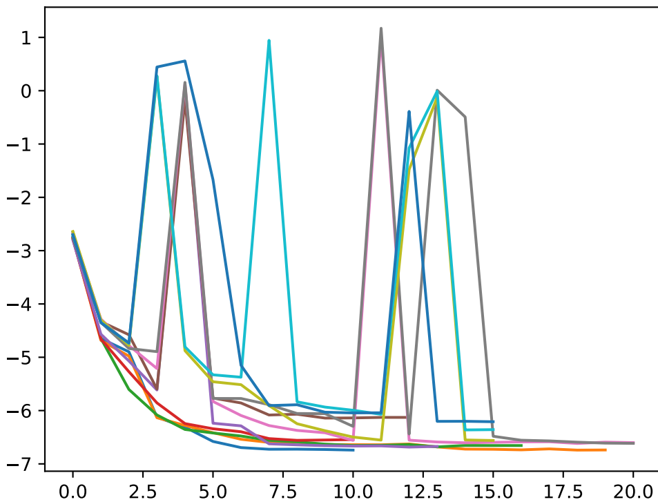
Exact derivative
