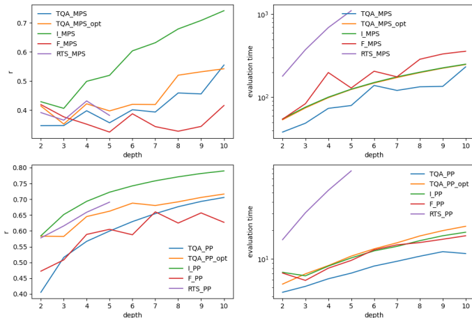
Figure: Results generated from a 106-node heavy-hex graph via the MPS(top row) and PP(bottom row) evaluators.
