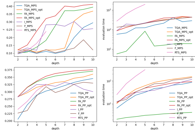
Figure: Results generated from a random 100-node 3-regular graph via the MPS(top row) and PP(bottom row) evaluators.
