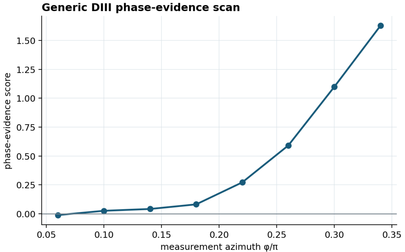
Figure 7. Generic DIII coarse evidence and selected refinement bracket. Interpretation limit: Finite widths and declared fit windows limit interpretation.
