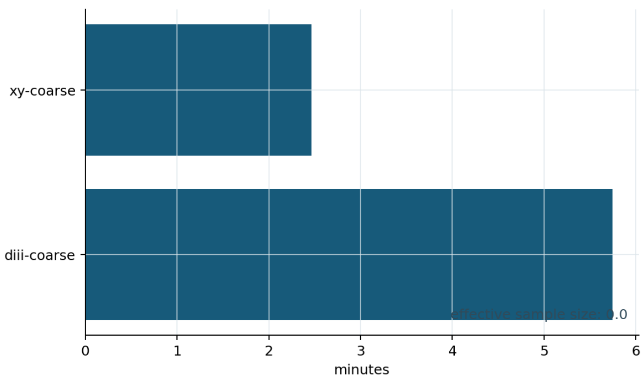
Figure 5. Runtime allocation and effective sample size.
