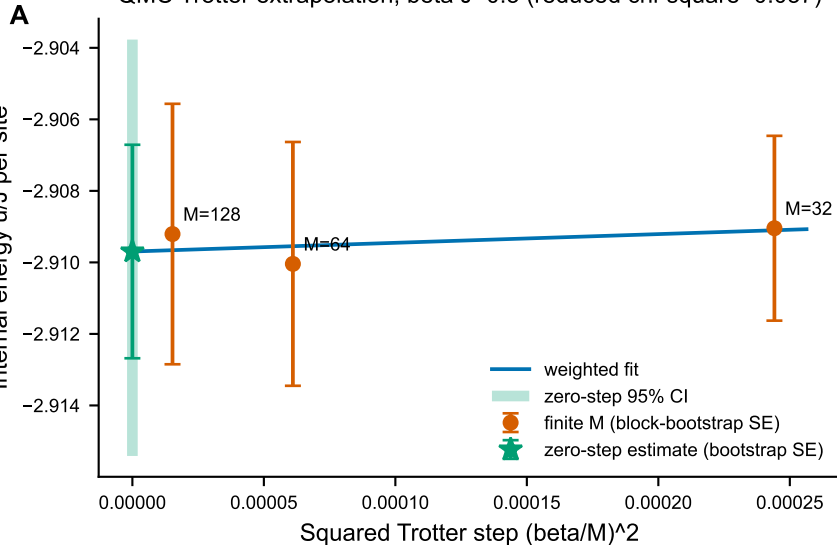
QMC Trotter extrapolation, beta J=0.5 (reduced chi-square=0.037)
