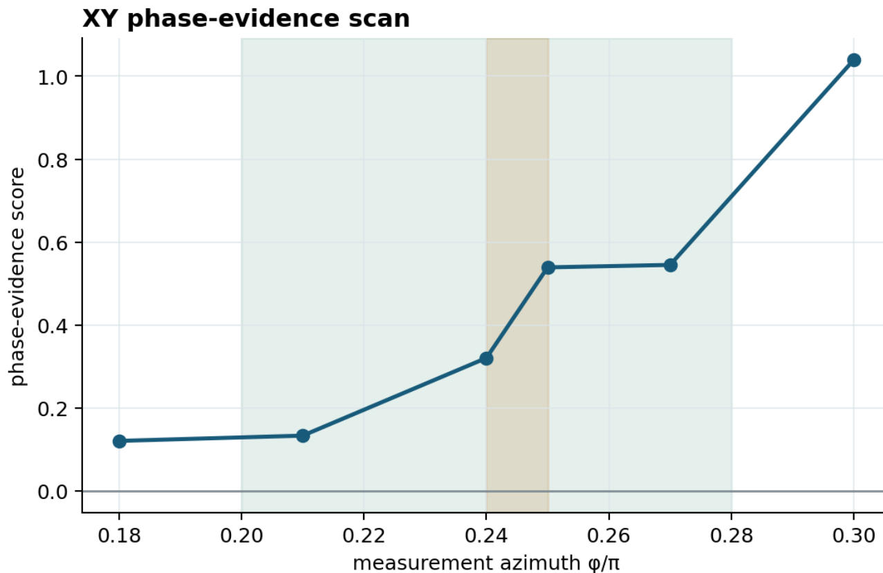
Figure 6. XY validation scan and declared reference window. Interpretation limit: Finite widths and declared fit windows limit interpretation.
