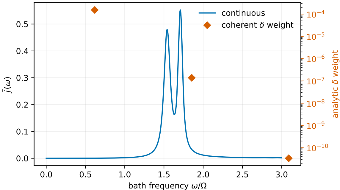
N=2 heat-current spectrum — Floquet-Markov/QRT
