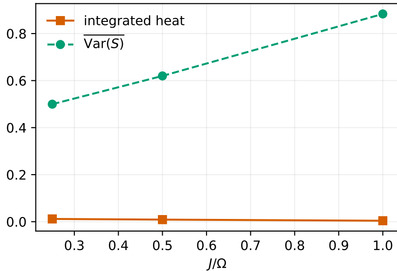
Heat and collective variance
