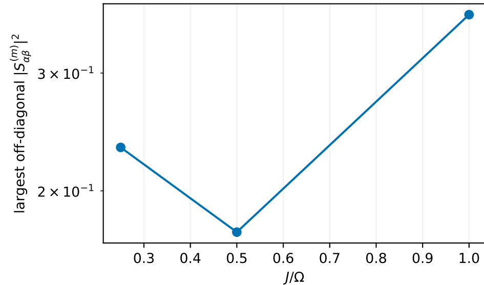
Floquet matrix-element diagnostic
