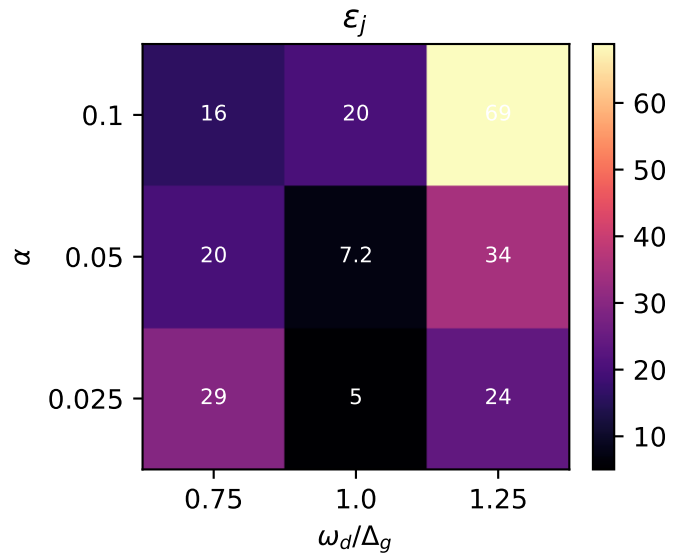
uniform TEMPO vs Floquet-Markov/QRT — N=2 interacting triplet calibration
