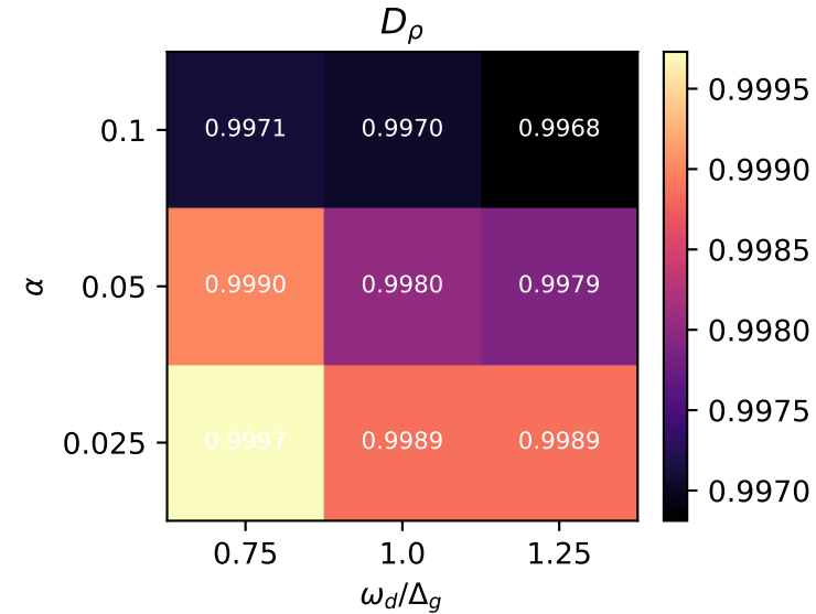
uniform TEMPO vs Floquet-Markov/QRT — N=2 interacting triplet calibration
