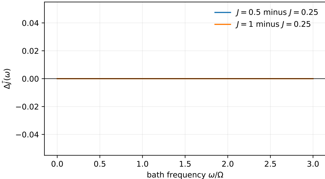
Reflection-odd heat spectrum: exact J -invariance check
