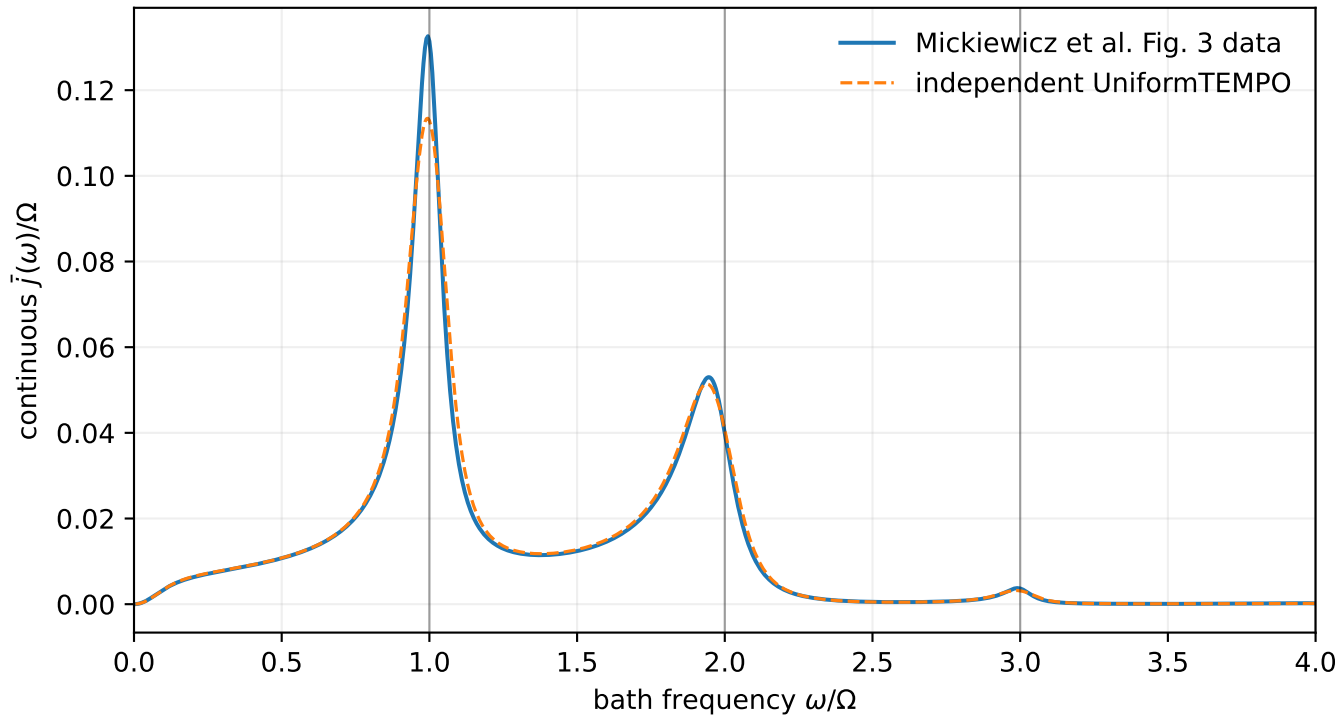
Fig. 3 bottom validation, \omega_d = 1\Omega
