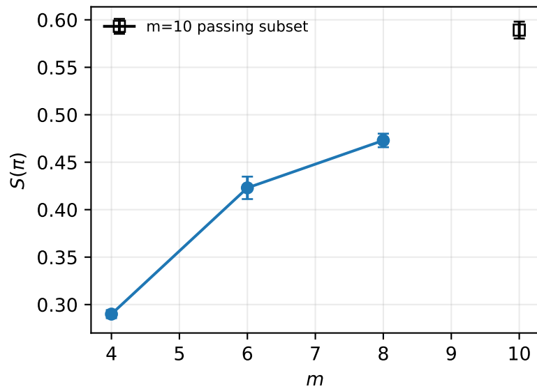
Numerical-only sentinel selection: g_B/g_A = 0.25 , t/g_A = 0.5 , \beta g_A = 4 Not thermodynamic phase evidence; m=10 marker uses 2/4 passing replicas
