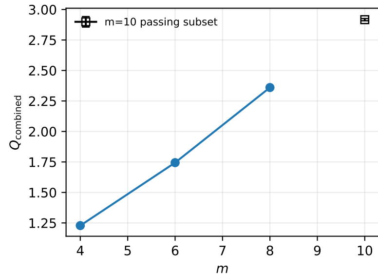
Numerical-only sentinel selection: g_B/g_A = 0.25 , t/g_A = 0.5 , \beta g_A = 4 Not thermodynamic phase evidence; m=10 marker uses 2/4 passing replicas
