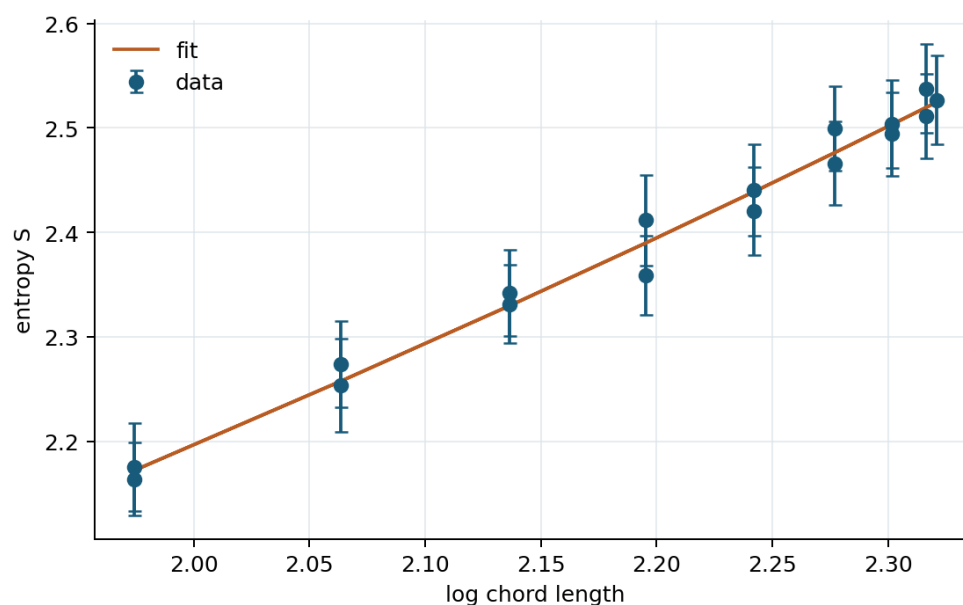
Figure 22. The central-interval entropy data are compared with the conformal chord form used to obtain c_{\text{eff}}^S(L) . Interpretation limit: A visually smooth chord fit does not remove cross-width extrapolation uncertainty or establish a DIII critical point.
