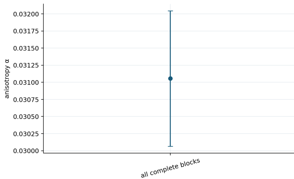
Figure 26. The frozen alpha estimate is 0.031056; the stability gate passed=False. Interpretation limit: Window sensitivity propagates directly into c_{\text{eff}}C and is therefore a required publication gate.
