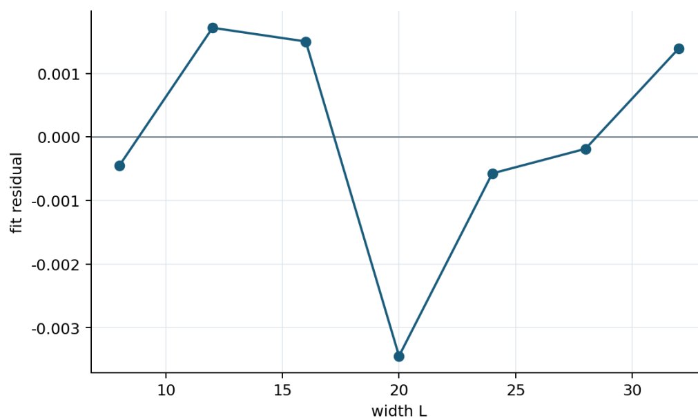
Figure 25. Residual structure tests whether the selected correction family absorbs the measured width dependence. Interpretation limit: Small residuals alone cannot rescue an unstable anisotropy calibration.
