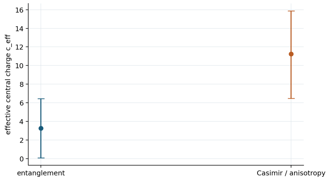
Figure 27. Entanglement gives 3.259733, whereas the Casimir-anisotropy route gives 11.251995. Interpretation limit: Their uncertainty bands do not satisfy the predeclared agreement test; the discrepancy is reported rather than averaged away.
