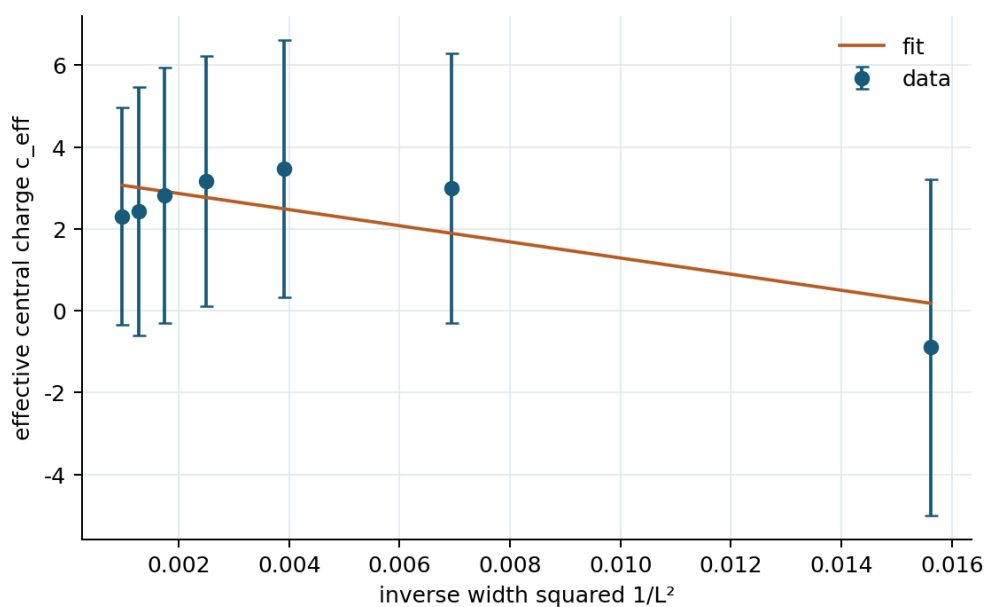
Figure 23. The intercept is 3.259733, with 95% interval [0.085659, 6.433808]. Interpretation limit: The interval is broad because individual-width slopes are noisy and strongly finite-size dependent.
