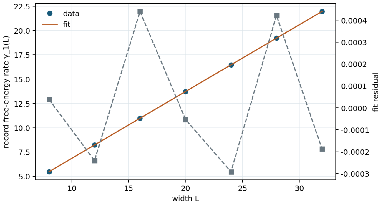
Figure 15. Casimir finite-size fit with residuals. Interpretation limit: Finite widths and declared fit windows limit interpretation.
