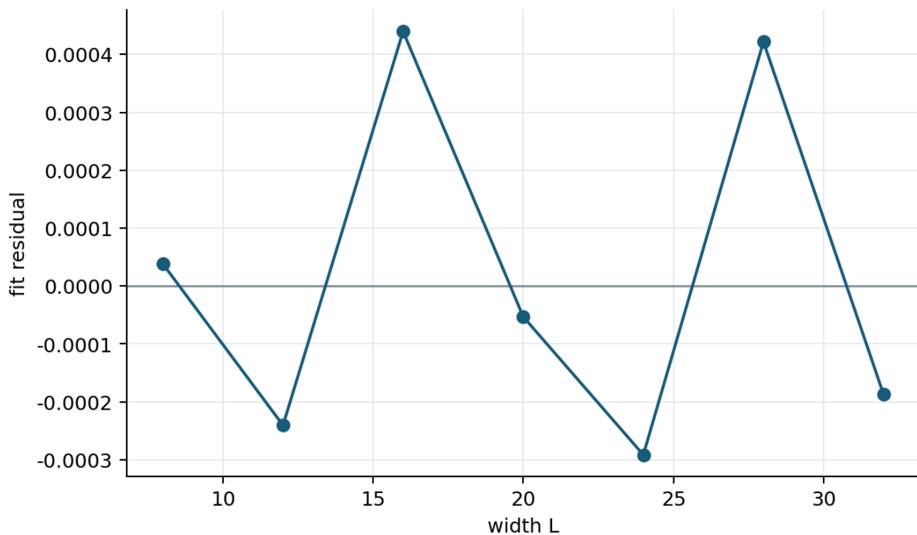
Figure 16. Residuals of the Casimir finite-size fit. Interpretation limit: Finite widths and declared fit windows limit interpretation.
