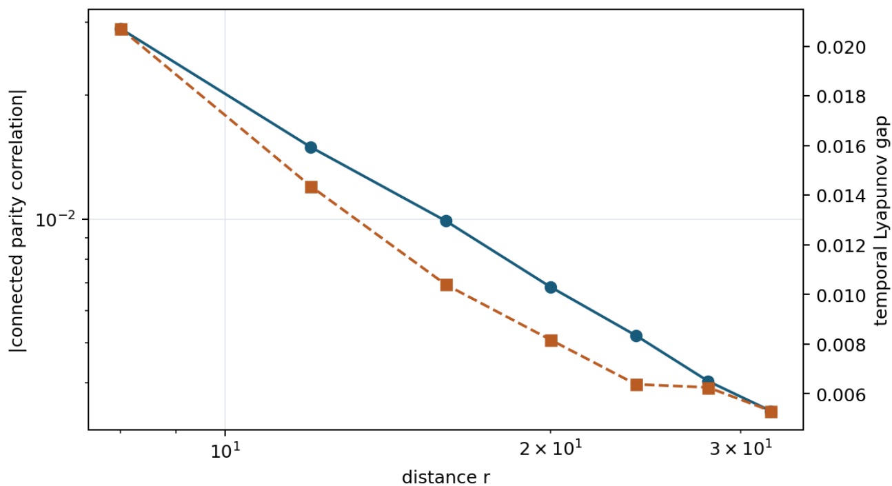
Figure 11. Spatial parity decay and temporal Lyapunov gaps. Interpretation limit: Finite widths and declared fit windows limit interpretation.
