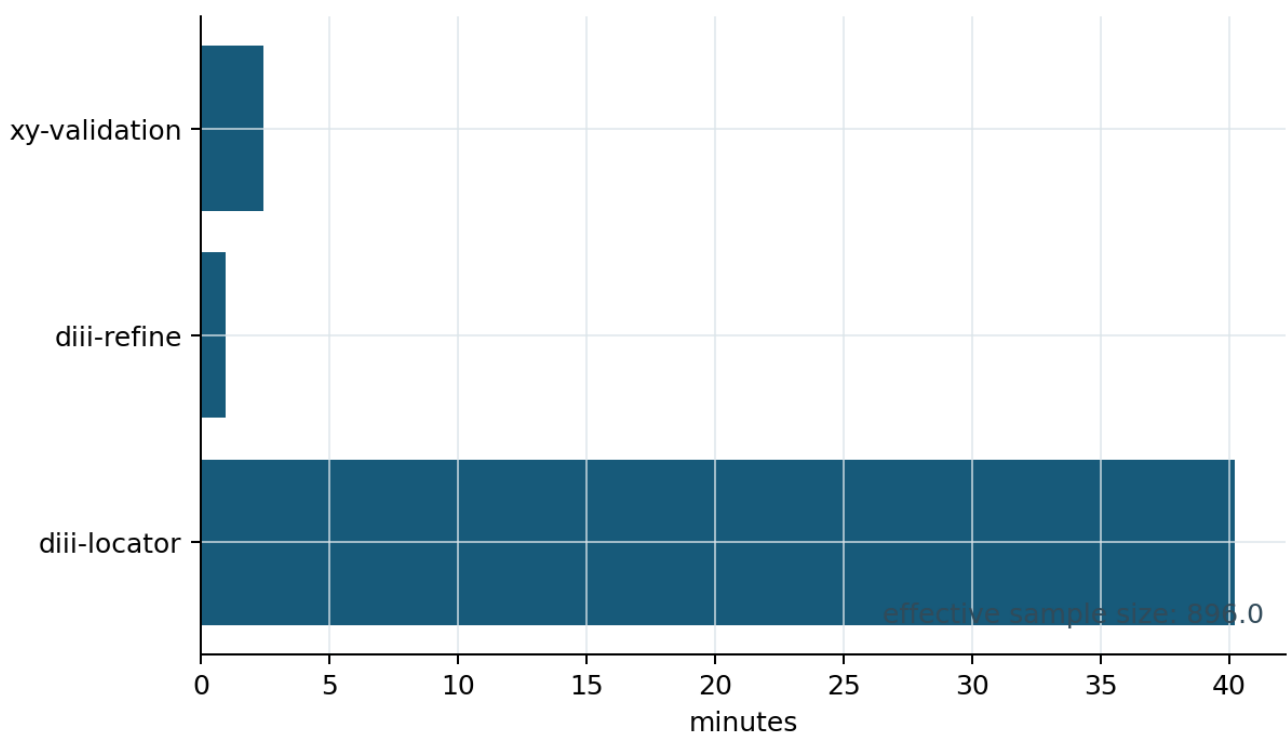
Figure 5. Runtime allocation and effective sample size.
