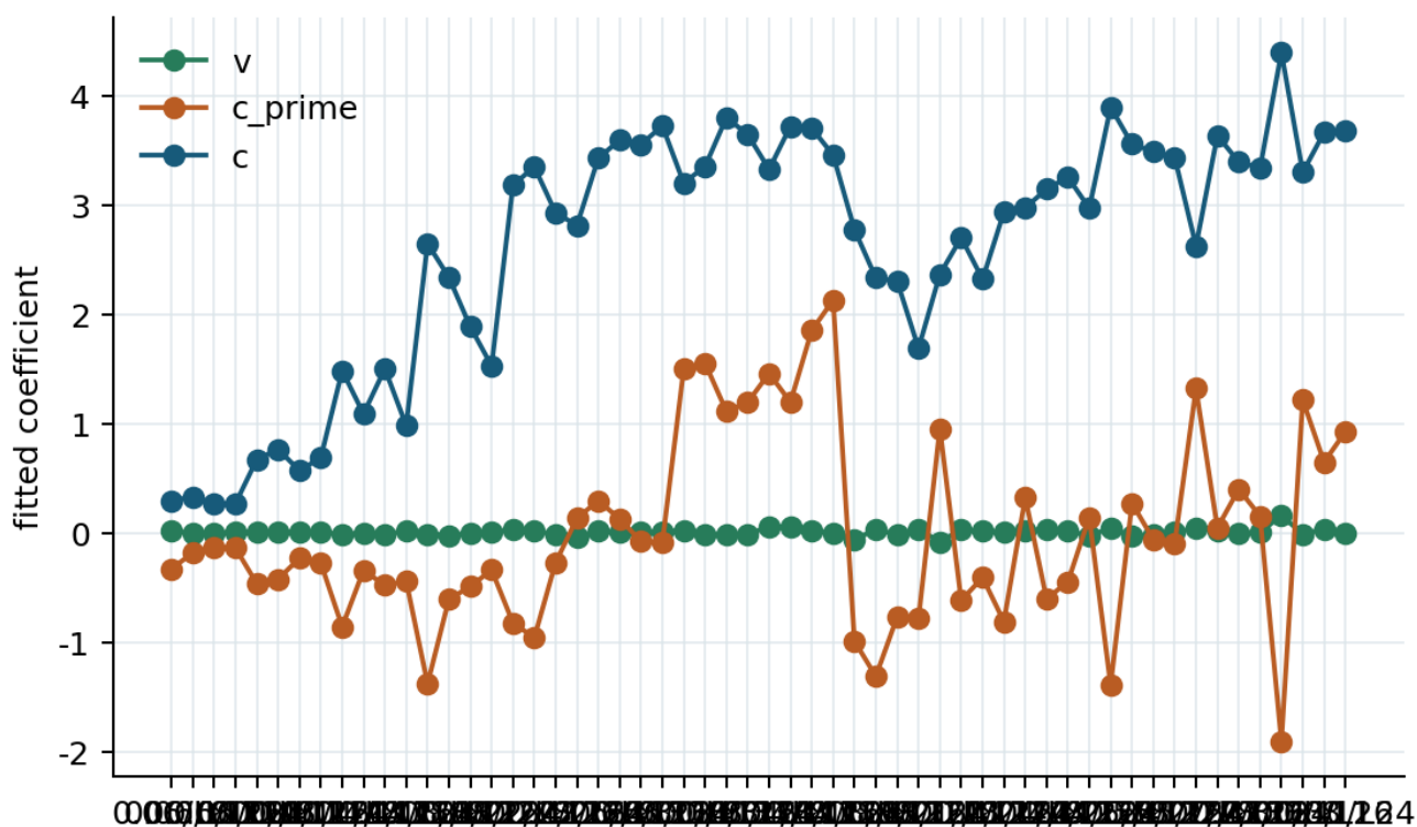
Figure 7. Generic DIII coarse evidence and selected refinement bracket. Interpretation limit: Finite widths and declared fit windows limit interpretation.
