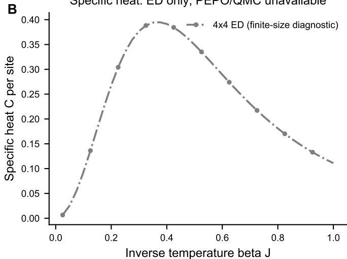
Figure 1 | Available thermodynamics at h/J=3 (lattice sizes shown explicitly)
