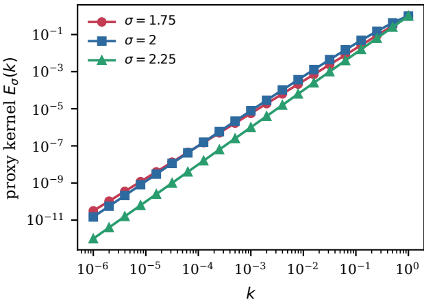
(a) Small-momentum kernels
