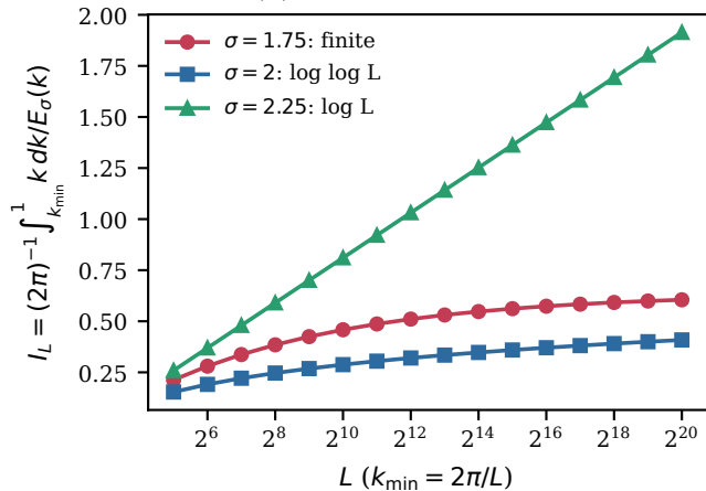
(b) Infrared accumulation
