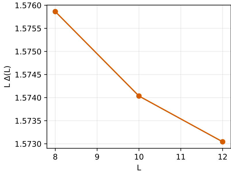
Periodic nearest-neighbor TFIM at \Gamma = 1
