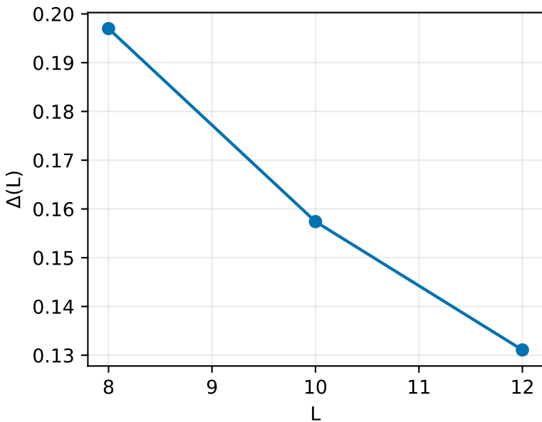
Periodic nearest-neighbor TFIM at \Gamma = 1
