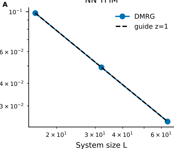
NN TFIM
