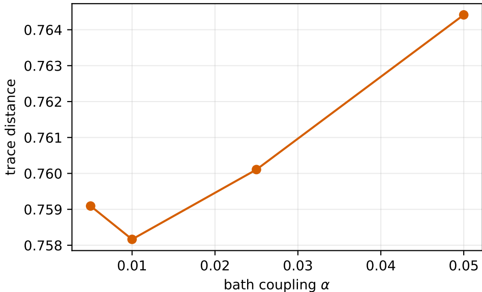
Finite-memory IF vs Floquet-Markov (both approximate)
