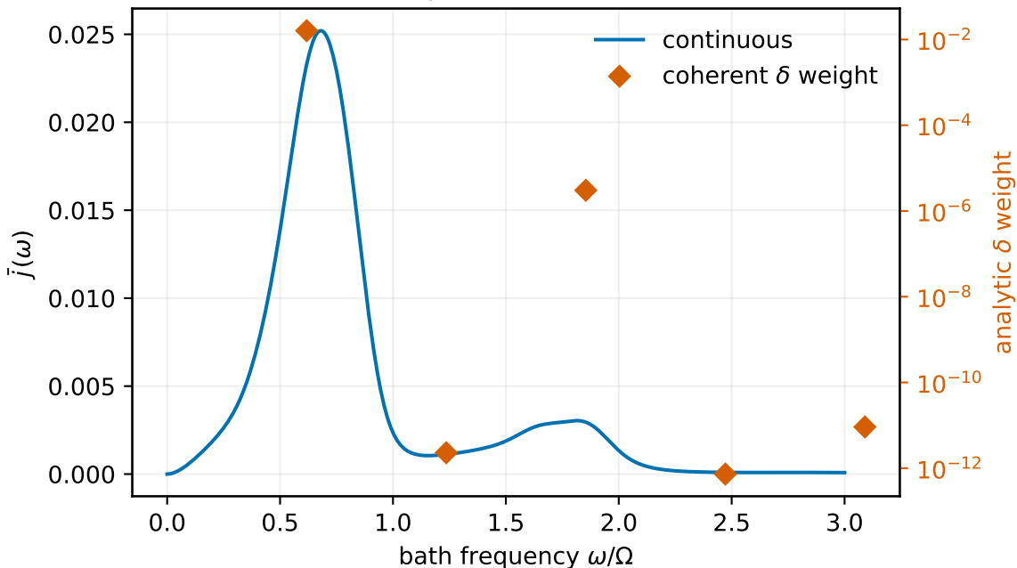
N=2 heat-current spectrum — PT-TEMPO multitime
