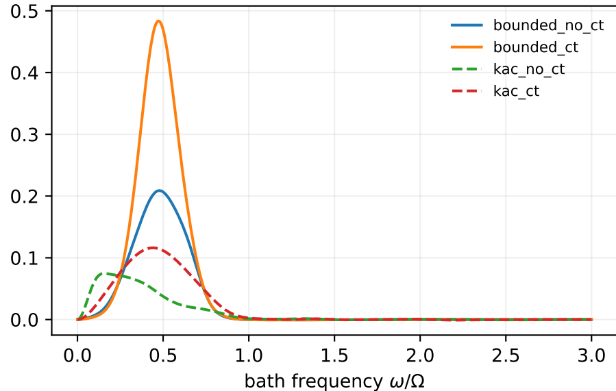
Diagnostic \bar{j}(\omega)/\eta^2
