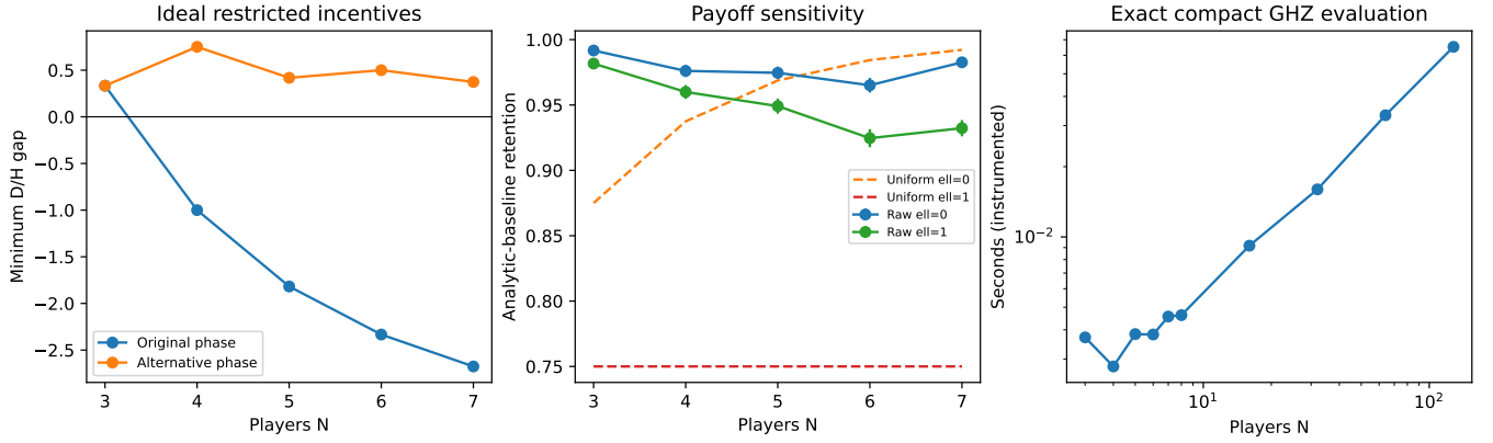
FIGURE 5. Journal-extension analyses. Left: minimum ideal Hawk/Dove deviation gap for the original and alternative cooperative phase branches, each in its stated restricted menu. Middle: retrospective raw fold-1 retention under the original and partial-conflict payoff rules for the recorded N = 3-7 run; error bars are 1.96 multinomial standard errors and exclude calibration drift. Uniform independent-outcome comparators are diagnostic, not equilibria. Right: exact compact GHZ payoff evaluation through N = 128 ; instrumented CPU time is a classical resource measurement, not hardware player-count scaling.
