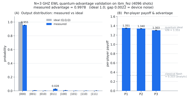
FIGURE 6. Hardware validation of the N=3 GHZ EWL quantum advantage on ibm_fez (IBM Heron r2). The validated (Q, Q, Q) circuit, with entangler J decomposed to 6 native \text{cz} gates, was executed with 4096 shots. (A) Measured output distribution over the eight computational-basis states (blue) versus the noiseless ideal (grey); error bars are binomial shot noise. 3911/4096 shots (95.5%) fall in |0 \dots 0\rangle , the ideal (Q, Q, Q) output. (B) Measured per-player payoff (blue) against the analytic classical-Nash baseline (0.333, noiseless) and the quantum ideal V/N = 1.333 ; error bars propagate shot noise. The measured mean payoff 1.331 gives advantage 0.9978 vs the ideal 1.0. Physical qubits \{136, 143, 142\} (calibration 2026-07-15): readout error 0.38–0.40%, \text{cz} error 136–143: 0.17%, 143–142: 0.23%.
