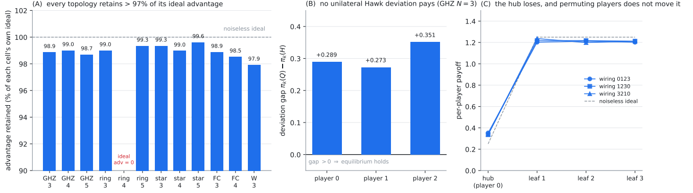
FIGURE 8. Multi-topology EWL batch on ibm_fez (job d9ia1pd0k0jc738jaqgg ), 49 pubs \times 4096 shots on one pinned qubit set, all predictions registered before submission. (A) Measured mitigated fold-1 advantage as a percentage of each cell's own noiseless advantage; the eleven nonzero-baseline cells retain 97.9–99.6%. ring N=4 carries no percentage because its noiseless advantage is exactly zero: its ideal circuit is deterministic on |1 \dots 1\rangle , so the +0.089 it measures is created by decoherence, and zero-noise extrapolation correctly pulls it back toward zero ( +0.037 ). (B) Unilateral Hawk deviation gaps \pi_k(Q, Q, Q) - \pi_k(H \text{ at } k) at GHZ N=3 : all three are positive, so no measured Hawk deviation pays; Dove deviations were not measured. (C) star N=4 per-player payoffs under three wirings. The hub earns \approx 0.34 while each leaf earns \approx 1.21 , and permuting players across physical qubits does not move the pattern: the disadvantage is locked to the graph position, not to the qubit.
