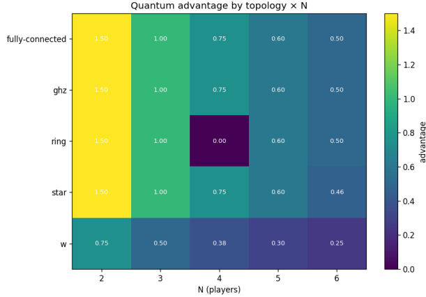
FIGURE 2. Circuit-relative payoff-gap heatmap across the (N, \text{topology}) grid at V=4, C=3 (mean per-player payoff of (Q_N, \dots, Q_N) minus the highest-mean circuit-evaluated restricted \{D, H\} equilibrium payoff). GHZ and fully connected hold the 3/N gap everywhere; the single dark cell is the ring at N=4 (gap exactly 0).
