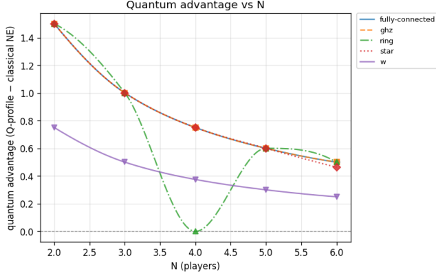
FIGURE 1. Zero-noise circuit-relative payoff gap of the fixed profile (Q_N, \dots, Q_N) , defined as its mean payoff minus the highest-mean circuit-evaluated restricted \{D, H\} equilibrium payoff, at \gamma = \pi/2 and V=4, C=3 . The 3/N gap (star markers) is attained by GHZ and fully connected at every recorded N ; the ring has zero gap at N=4 ; the star shows a weaker N=6 value (0.463 vs. 0.5); and W tracks below throughout. Filled markers indicate that the profile passes the restricted \{D, H, Q_N\} deviation check, which depends on topology.
