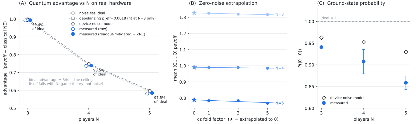
FIGURE 7. Cross-calibration aggregate of the N -player GHZ EWL quantum advantage on ibm_fez (IBM Heron r2): three executions spanning two distinct provider calibrations , all on the same physical chain [59, 75, 74, 73, 79], 4096 shots each. Executions sharing a calibration stamp are averaged into one point before the spread is taken, because two runs under one calibration are one sample rather than two; the two epochs are 2026-07-16 08:30:13 (two executions) and 2026-07-26 13:29:01 (one). A fourth execution exists on chain [20, 21, 22, 23, 24] and is deliberately excluded here: pooling it would confound calibration drift with a change of physical qubits. Table 2 reports the registration-source execution alone. (A) Measured cooperative-profile advantage (mean (Q, \dots, Q) payoff minus the analytic noiseless classical-Nash payoff) at N = 3, 4, 5 : raw (open) and readout-mitigated + ZNE (filled), against the noiseless ideal (1.0, 0.75, 0.6), the device noise-model prediction (diamonds), and a single-parameter depolarizing model with p_{\text{eff}} = 0.0018 fitted to the N=3 point alone; its N=4, 5 values are predictions, not fits. The ideal, device-model and depolarizing curves are the registration anchor's rather than run averages, so the registered p_{\text{eff}} is quoted unchanged. Error bars are the sample standard deviation across the two calibration epochs, a genuine cross-calibration estimate unlike the within-epoch spread reported in earlier drafts, and still exclude the within-run multinomial and weighted-fit standard errors, so they are a lower bound on total uncertainty. (B) ZNE mechanics: readout-mitigated payoff vs cz fold factor ( \lambda = 1, 3, 5 ) with the weighted linear fit extrapolated to \lambda = 0 (stars). (C) Ground-state probability P(|0 \dots 0\rangle) : the all-zero target-state population decays several times faster than the advantage because the mean-payoff observable is first-order insensitive to single bit-flips from |0 \dots 0\rangle . (Q, \dots, Q) passes the restricted-menu pure-Nash check only at N=3 among the plotted genuinely multiplayer cases; at N=4, 5 the profile is the cooperative quantum protocol, not an equilibrium.
