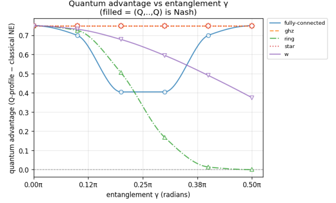
FIGURE 3. Circuit-relative payoff gap versus entanglement angle \gamma at N=4 ( V=4, C=3 , noiseless). GHZ and star hold 0.75 flat; fully connected dips and recovers; W decays monotonically; and ring falls to zero at \gamma = \pi/2 . Data: results/gamma-sweep/N4.
