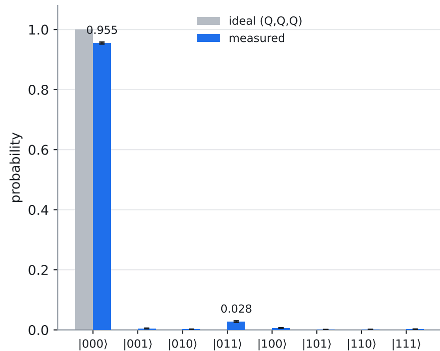
(A) Output distribution: measured vs ideal
