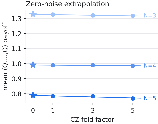
Fig. 8. Zero-noise extrapolation of the readout-mitigated mean payoff in the registration-source execution at N = 3, 4, 5 . Points at CZ fold factors 1, 3, 5 carry within-run payoff standard errors; weighted linear fits extrapolate to zero fold factor (stars). The N = 4, 5 profiles are cooperative protocols, not restricted pure-Nash equilibria.
