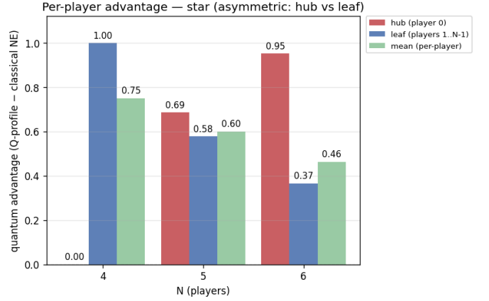
Fig. 4. Star-topology per-player circuit-relative payoff gap (hub player 0 vs. each leaf) at \gamma = \pi/2 , V=4, C=3 , noiseless, for N = 4 \dots 6 . Labels show gaps to two decimal places, including the numerically zero hub gap at N=4 ; green bars show the per-player mean. Data: results/n-scaling-advantage/2026-07-19T0901Z.
